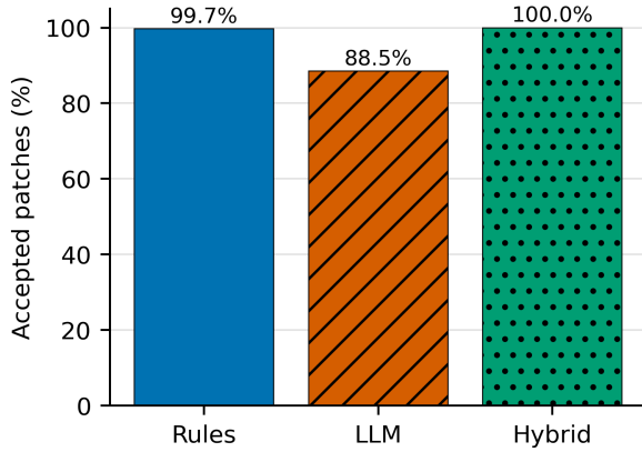
Figure 4. Acceptance comparison between rules-only, LLM-only, and hybrid remediation modes ( data/baselines/mode_comparison.csv ).
