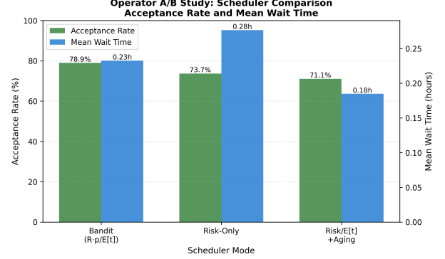
Figure 5. Simulated scheduler replay comparing bandit scheduling against baseline modes. Dual-axis chart shows acceptance rate (green bars) and mean wait time (blue bars) across 247 scheduler-arm assignments over a 152-item toy queue ( data/operator_ab/summary_simulated.csv ).
