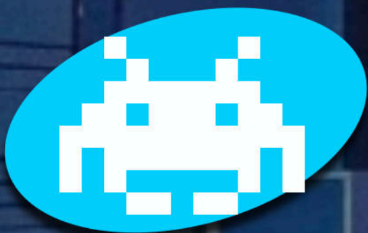
Monitor-Bot
