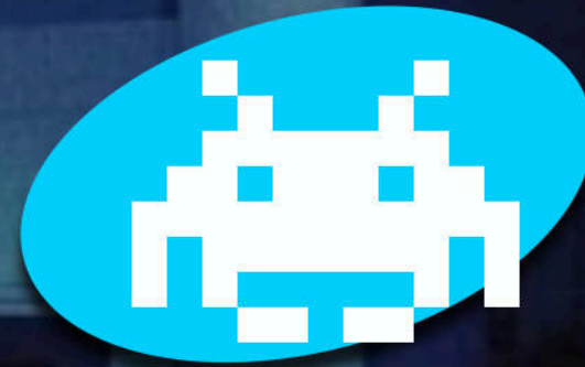
Monitor-Bot
