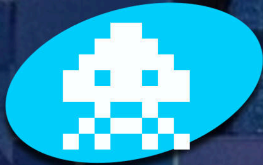
Buy-Bot
