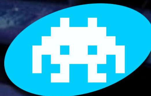
Sell-Bot
