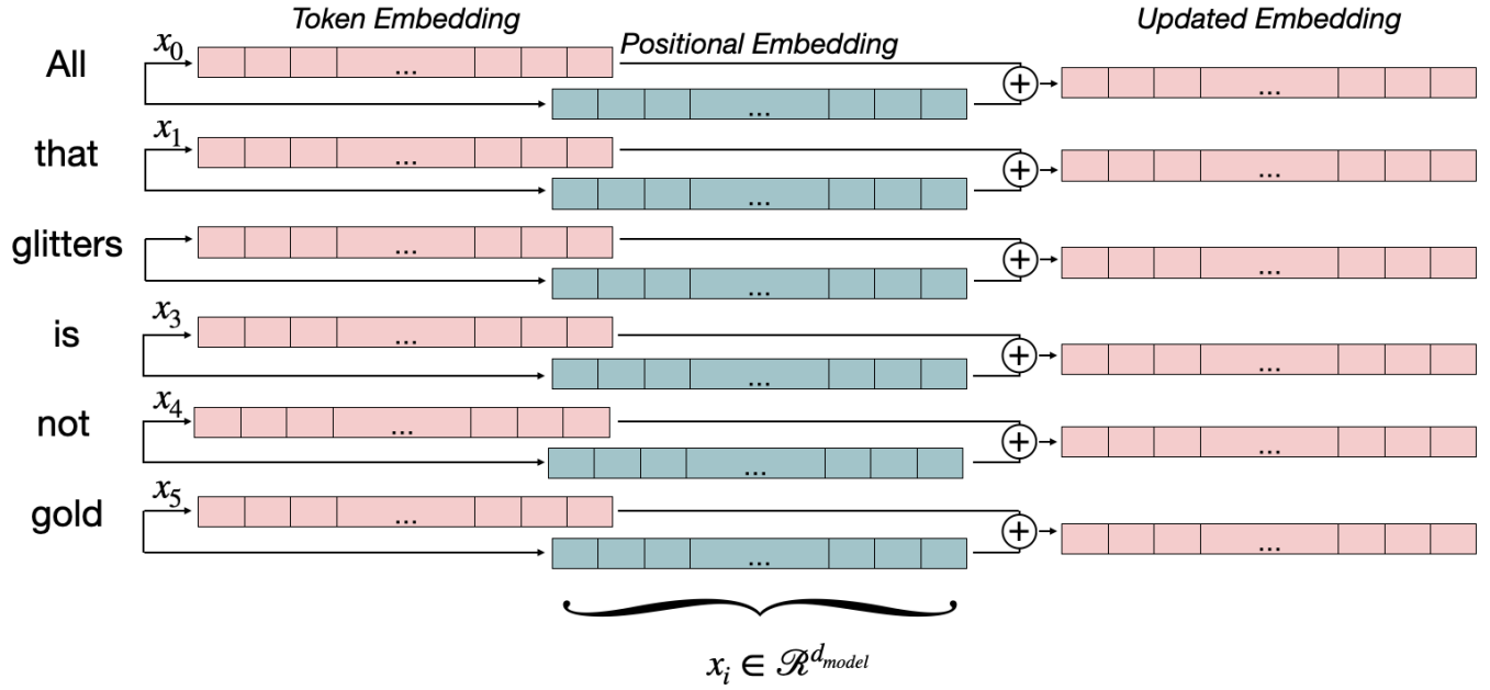
Figure 10: A token’s embedding vector is “plucked” from the token embedding matrix, and its corresponding positional vector is also “plucked” from the positional embedding matrix. These two vectors are added together and are the first update in the transformer architecture that adds context to token embeddings vectorial representation.
