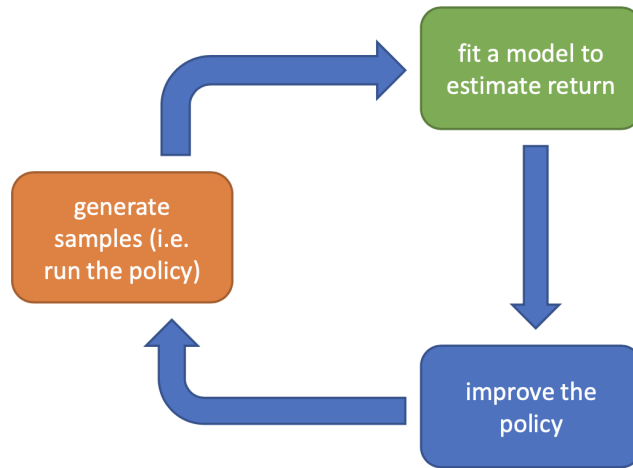
Figure 11: REINFORCE algorithm
