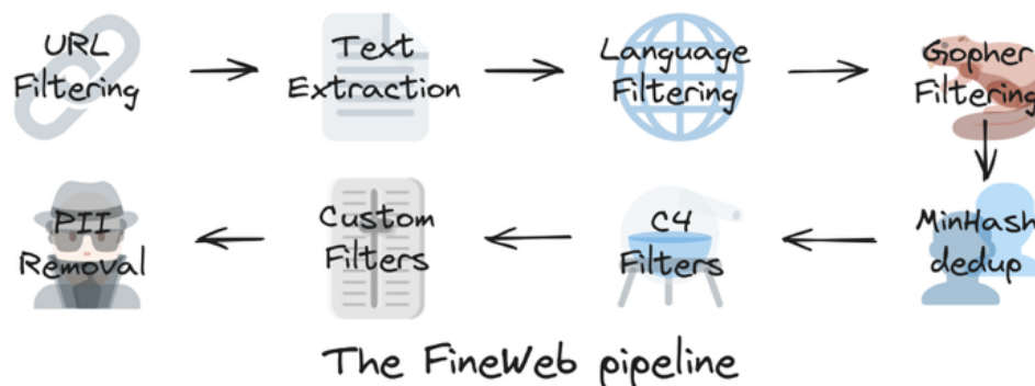
Figure 8: The Hugging Face process for filtering Common Crawl.
