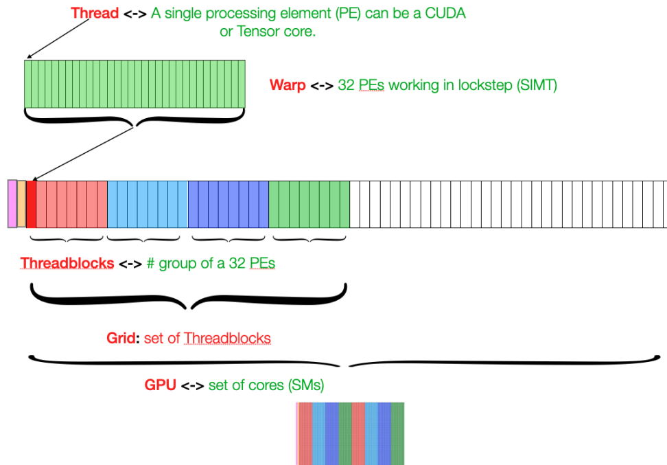
Figure 15: A visual representation of The relationship between hardware and software terminology. The red represents the software abstractions and the green represents the hardware terminology.
