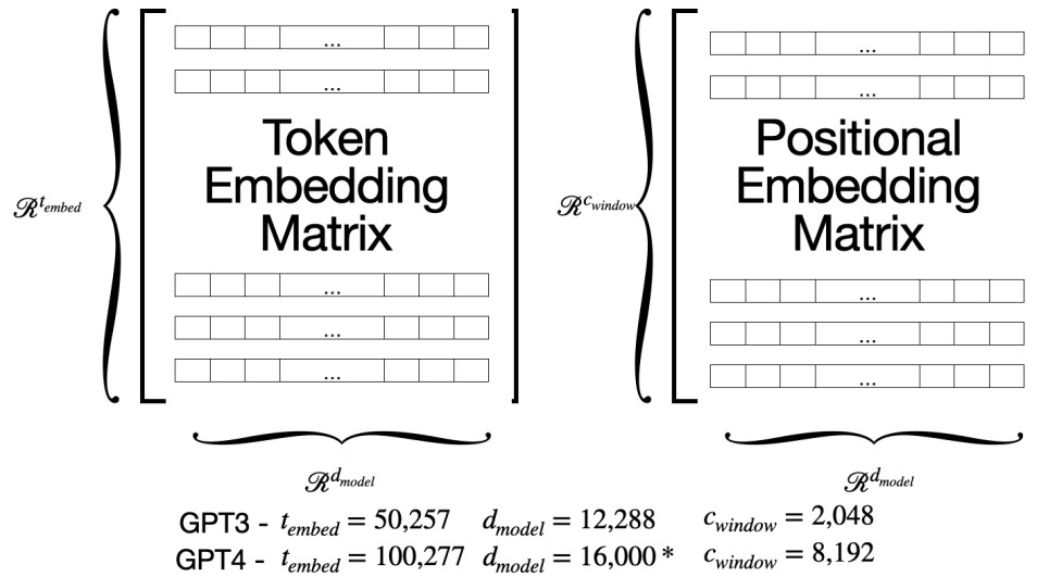
Figure 9: The embedding matrix dimensions.
