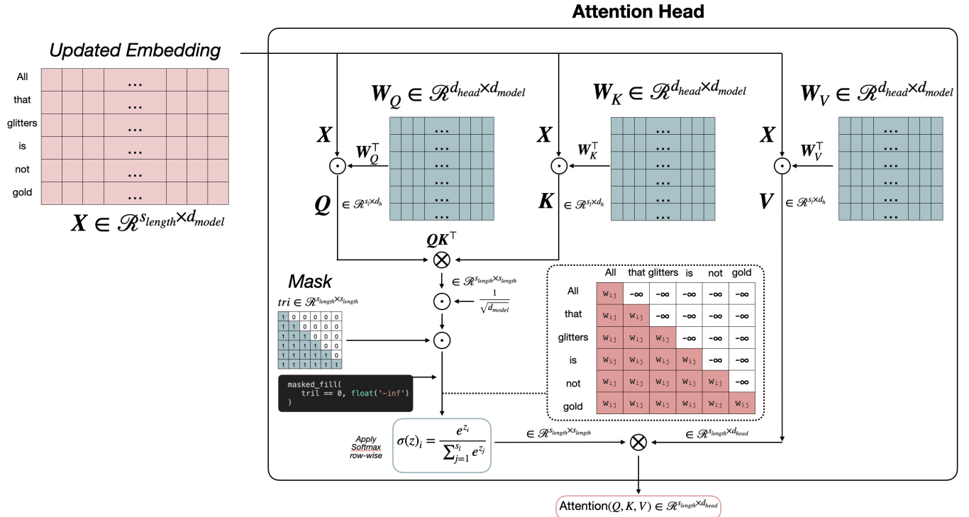
Figure 11: A single attention head.
