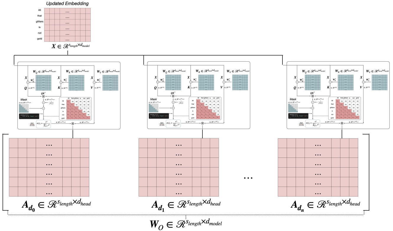
Figure 12: Multiple heads of attention.
