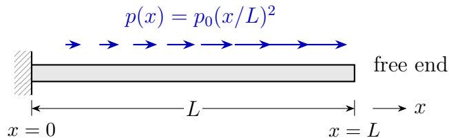
Figure 2.1: Fixed-free bar subjected to a nonuniform axial load.
