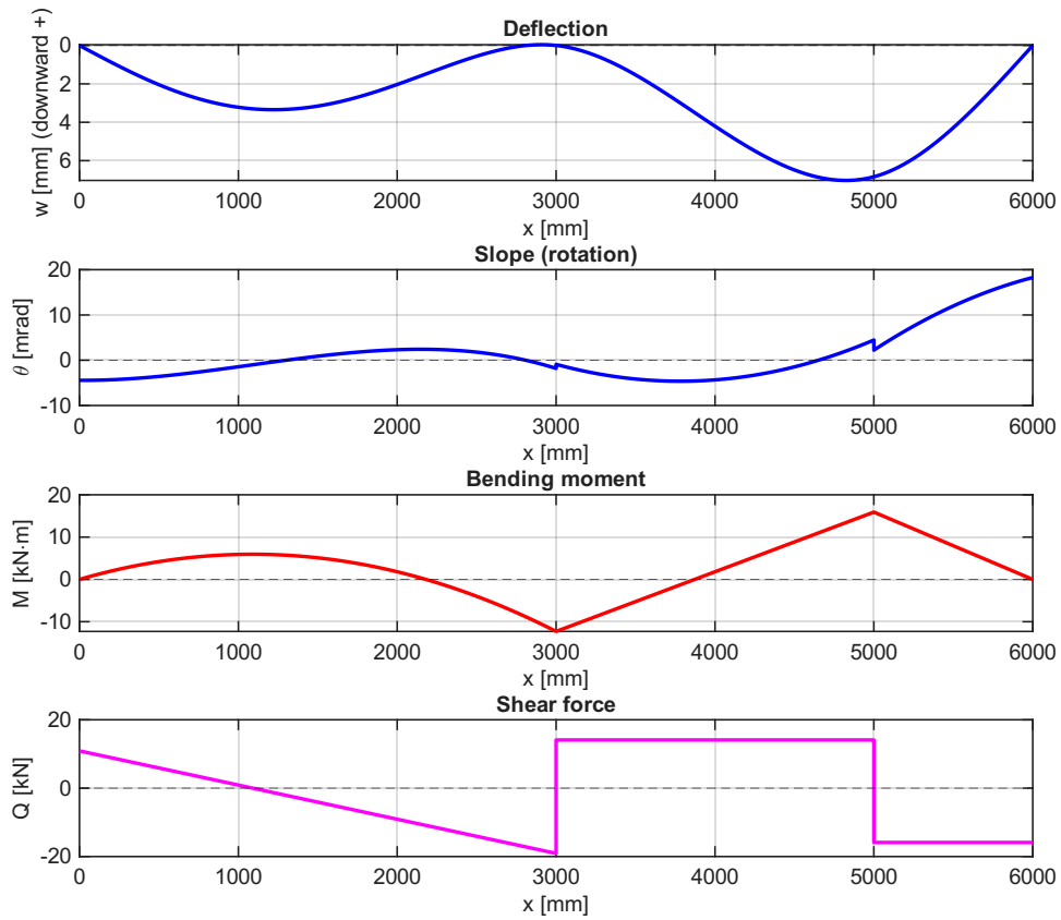
Figure 5.5: Continuous beam internal fields. Top to bottom: deflection (downward positive), slope, bending moment (sagging positive), shear force. Key values: w_3 = 6.84 \text{ mm} (downward), M_{\max} = +15.90 \text{ kN m} (sagging at node 3), M_{\min} = -12.29 \text{ kN m} (hogging at node 2).
