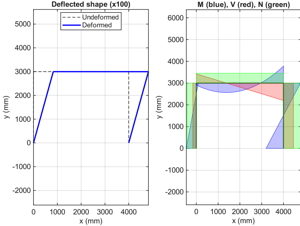
Figure 6.4: Portal frame results: deflected shape (left, displacements magnified \times 100 ) and internal force diagrams (right) for bending moment (blue), shear (red), and axial force (green).
