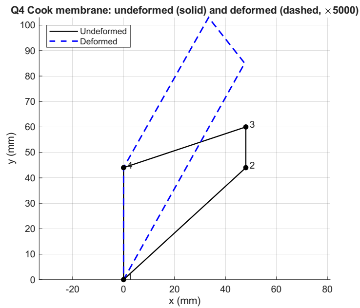
Figure 7.5: Cook membrane: undeformed (solid) and deformed shape (dashed, magnified \times 5000 ). Both right-edge nodes deflect vertically; the tapered geometry induces small lateral movement.
