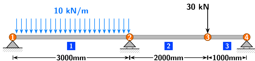
Figure 5.4: Three-element continuous beam. Distributed load q = 10 N/mm on element 1; concentrated load P = 30 kN at node 3. Pin support at node 1; rollers at nodes 2 and 4.
