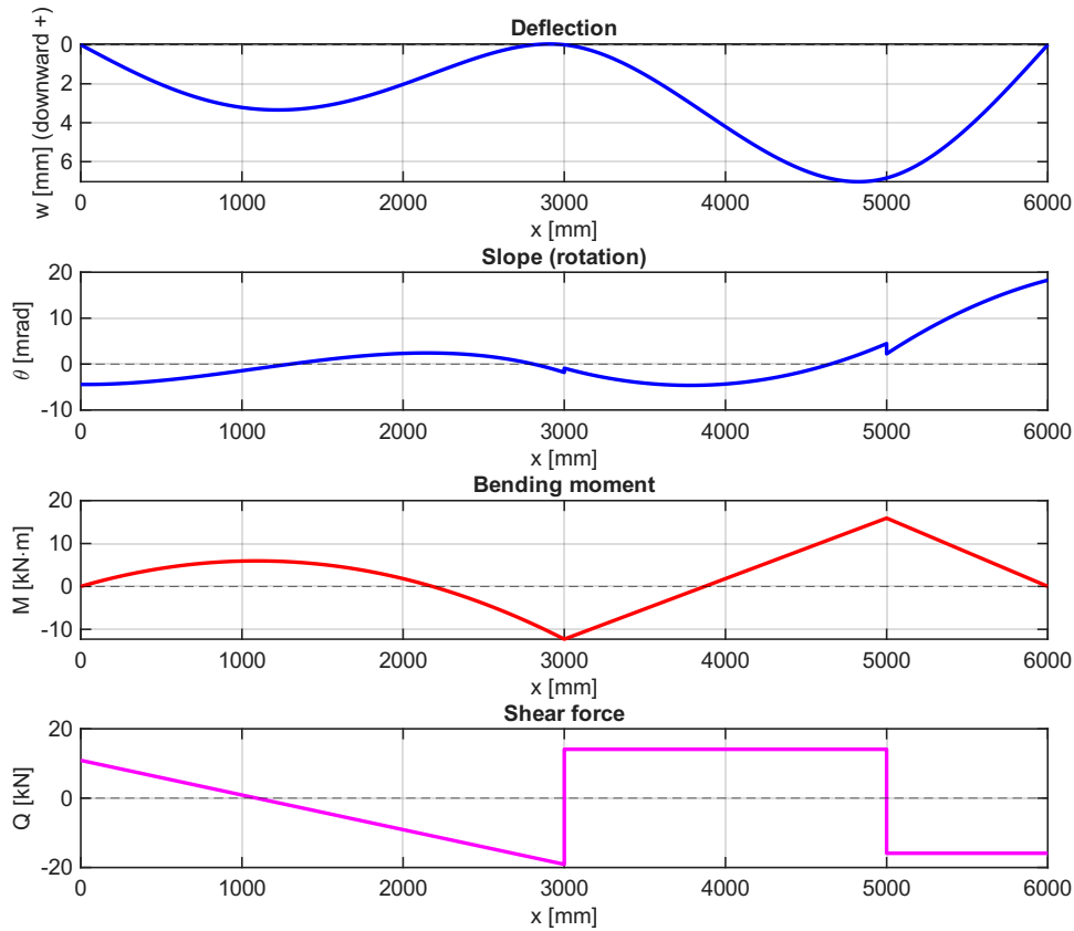
Figure 5.4: Continuous beam internal fields. Top to bottom: deflection (downward positive), slope, bending moment (sagging positive), shear force. Key values: w_3 = 6.84 \text{ mm} (downward), M_{\max} = +15.90 \text{ kN m} (sagging at node 3), M_{\min} = -12.29 \text{ kN m} (hogging at node 2).
