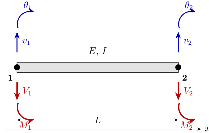
Figure 5.1: Two-node Euler-Bernoulli beam element. Transverse displacements v_1, v_2 (blue, upward positive) and rotations \theta_1, \theta_2 (blue, CCW positive) are the DOFs. End shear forces V_1, V_2 and bending moments M_1, M_2 (red) are the conjugate nodal forces.
