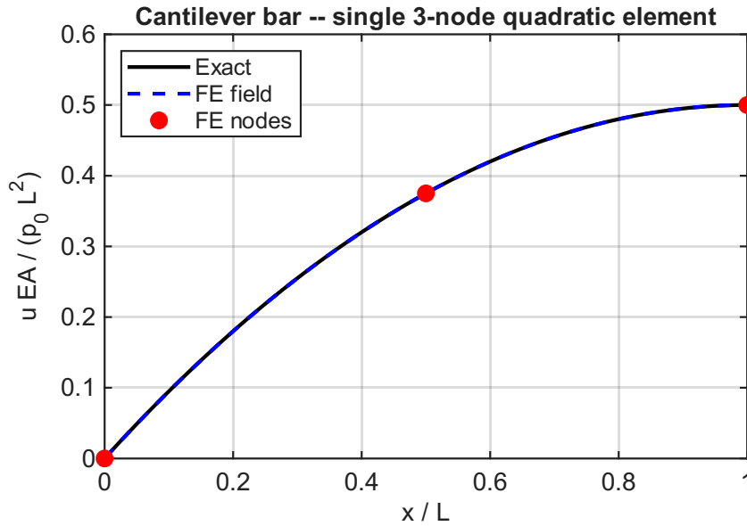
Figure 3.9: Cantilever bar under uniform axial load, single 3-node quadratic element. The FE displacement field (blue dashed) overlays the analytical solution (black solid); red markers show the three FE nodal values. Generated by Section A.4.
