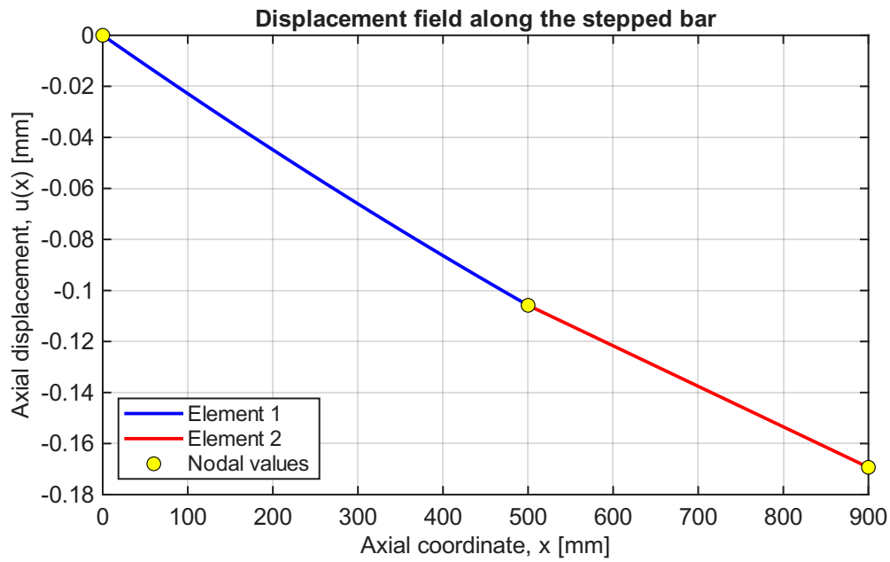
Figure 3.5: Displacement field u(x) along the stepped bar.
