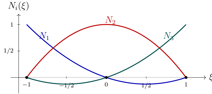
Figure 3.7: Quadratic Lagrange shape functions on the parent domain \xi \in [-1, 1] . Each N_i equals 1 at its own node and 0 at the others; the three sum identically to one. The end-node functions N_1 and N_3 dip slightly below zero between \xi = \pm 1/2 and the opposite end, reaching a minimum of -1/8 .
