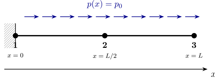
Figure 3.8: Cantilever bar under uniform axial load p_0 , modelled by a single 3-node quadratic element. Nodes 1, 2, 3 lie at x = 0, L/2, L .
