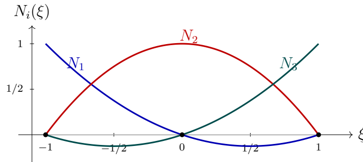
Figure 3.8: Quadratic Lagrange shape functions on the parent domain \xi \in [-1, 1] . Each N_i equals 1 at its own node and 0 at the others; the three sum identically to one. The end-node functions N_1 and N_3 dip slightly below zero between \xi = \pm 1/2 and the opposite end, reaching a minimum of -1/8 .
