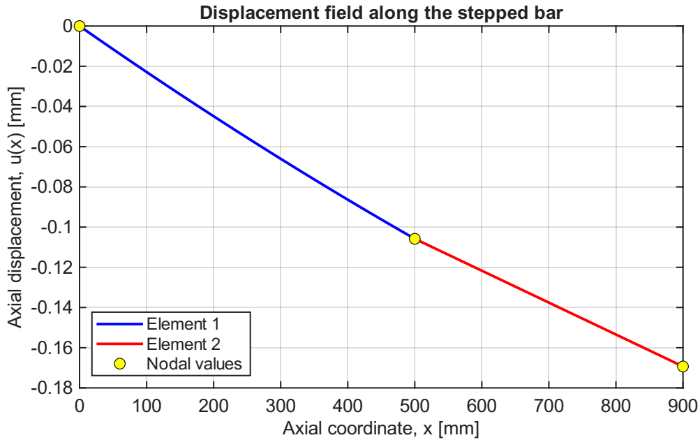
Figure 3.6: Displacement field u(x) along the stepped bar.
