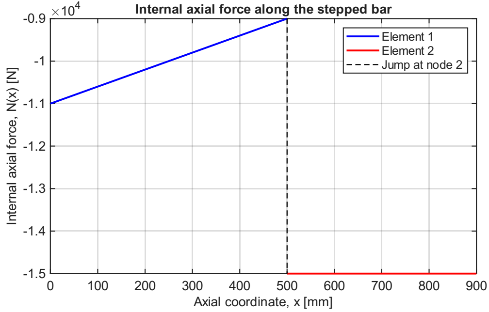
Figure 3.7: Internal axial force N(x) along the stepped bar. The discontinuity at x = 500 mm corresponds to the +6 kN concentrated force applied at node 2.
