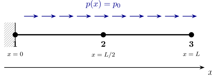
Figure 3.9: Cantilever bar under uniform axial load p_0 , modelled by a single 3-node quadratic element. Nodes 1, 2, 3 lie at x = 0, L/2, L .
