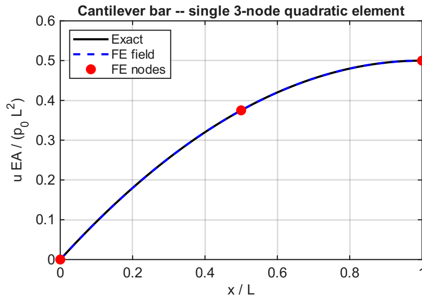
Figure 3.10: Cantilever bar under uniform axial load, single 3-node quadratic element. The FE displacement field (blue dashed) overlies the analytical solution (black solid); red markers show the three FE nodal values. Generated by Section A.4.
