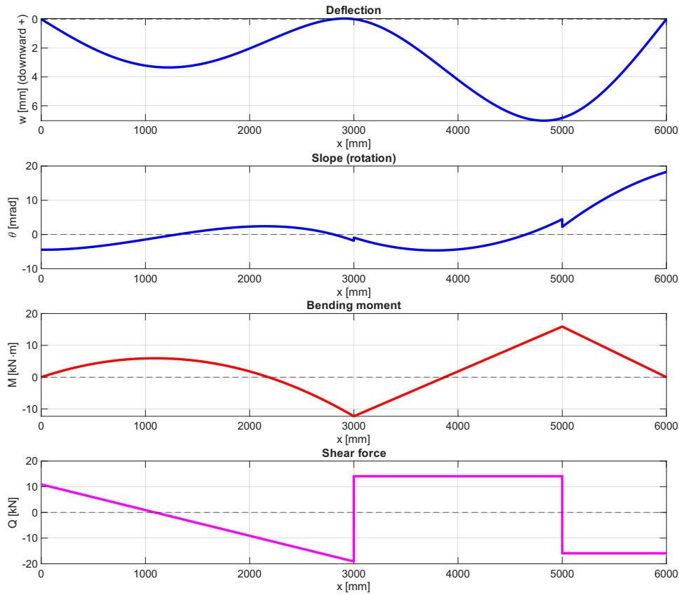
Figure 5.4: Continuous beam internal fields. Top to bottom: deflection (downward positive), slope, bending moment (sagging positive), shear force. Key values: w_3 = 6.84 mm (downward), M_{\max} = +15.90 kN m (sagging at node 3), M_{\min} = -12.29 kN m (hogging at node 2).
