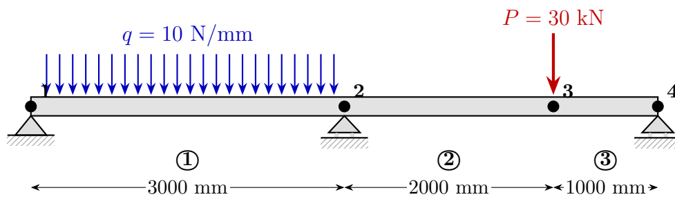
Figure 5.4: Three-element continuous beam. Distributed load q = 10 N/mm on element 1; concentrated load P = 30 kN at node 3. Pin support at node 1; rollers at nodes 2 and 4.
