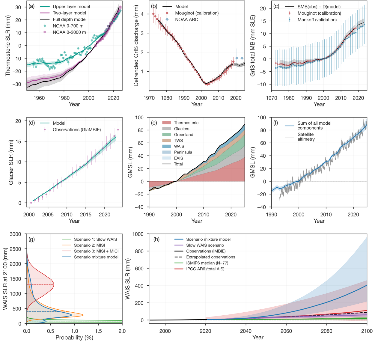
Figure 2: Model calibration, validation, and WAIS uncertainty. (a) Two-layer energy balance model fitted jointly to NOAA thermosteric sea level at 0–700 m (1957–2025) and 0–2000 m (2005–2025). (b) Greenland ice discharge modeled as a cumulative time-delay response to subsurface ocean warming ( \delta = 5 yr, R^2 = 0.995 ). Calibration data (Mouginitot et al. (2019) [34], filled circles) and withheld validation data (NOAA Arctic Report Card, diamonds) both fall within the 90% credible interval. (c) Global glacier contribution fitted to GlaMBIE consensus observations (2000–2023) using a linear temperature-driven model ( R^2 = 0.995 ). Grey band shows the 90% credible interval. (d,e) Budget closure: temperature-forced component hindcast (stacked) compared with NASA altimetry and reconstructions. The component sum closes the 2000–2025 budget to within 6%. (f) WAIS: IMBIE satellite observations (black) compared with the ISMIP6 ensemble median and interquartile range (green; [35]), our full scenario mixture (blue), the stable-WAIS scenario (purple), and IPCC AR6 total Antarctic projection (red).
