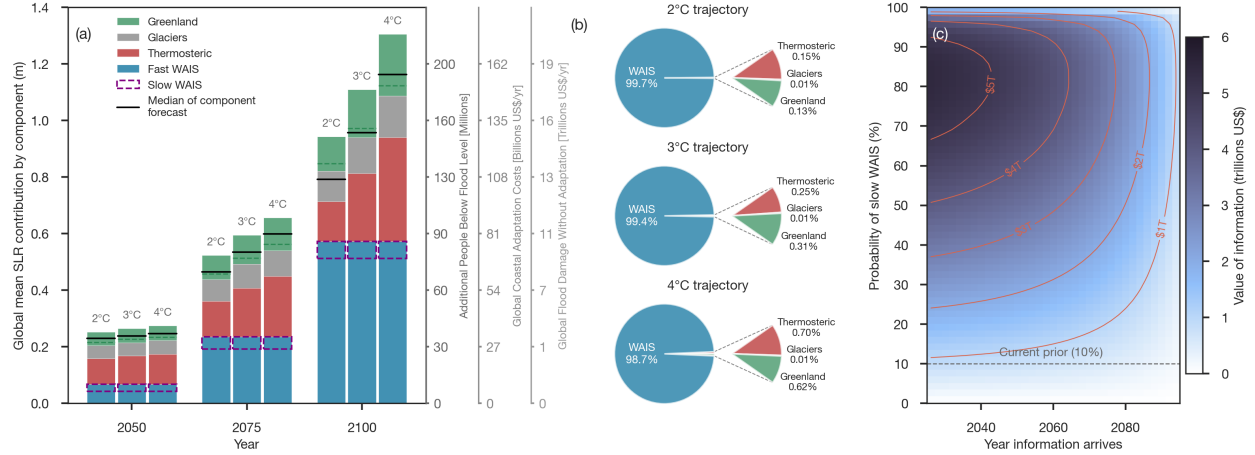
Figure 4: Component contributions, variance decomposition, and value of information. (a) 21st century mean GMSLR contribution by component at 2050, 2075, and 2100 for 2°C, 3°C, and 4°C warming trajectories. WAIS (bottom, blue) is emission scenario-invariant. All other components are emission-sensitive, and the value of emissions reduction can be traced by the stack heights and median values (black lines). Dashed purple boxes show the slow WAIS only scenario. Green dashed lines within Greenland bars partition discharge anomaly (below) from SMB anomaly (above). Gains in EAIS approximately offset losses in Peninsula, so we omit both. Right-hand axes show corresponding societal impacts as in Fig. 3. (b) Variance-fraction pie charts at 2100 for each warming trajectory. WAIS accounts for 97–99% of total forecast variance. Fan breakouts show the non-WAIS contributions. (c) Financial value of resolving WAIS uncertainty as a function of when information arrives and the probability of slow WAIS decline. Dashed line marks the current prior on WAIS Scenario 1 (10%). Contours and colormap in trillions US$ based on coastal adaptation costs (Supplemental Material).
