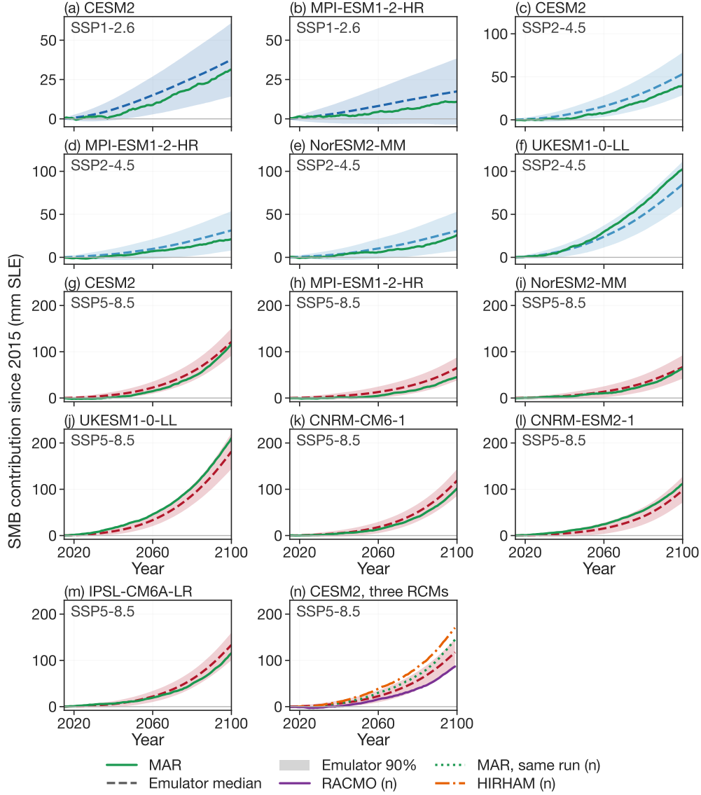
Figure S8: Greenland SMB projections of regional climate models against the emulator, 2015–2100. (a–m) Cumulative SMB contribution since 2015 of each MARv3.12 scenario run ( Boberg et al. , 2026) (green), relative to the 1995–2005 mean of that GCM’s history run, with the prediction of the emulator fitted to the other six GCMs and driven by the withheld GCM’s GMST (dashed median and shaded 90% range, colored by scenario). The range includes the spread of the six GCMs, the coefficient uncertainty, autoregressive weather noise, and the weather noise of the 1995–2005 anchor, and the values at 2100 are those of Fig. S7. (n) RACMO2.3p2 ( Noël et al. , 2021) (purple) and MAR (green dotted), both forced by a CESM2 SSP5-8.5 branch run, and HIRHAM (orange dash-dot), forced by CESM2 r1i1p1f1 under SSP5-8.5, all from Glaude et al. (2024), integrated over the contiguous ice sheet and taken relative to their own 1995–2005 means. RACMO ends in 2099. The emulator in (n) is fitted to the six GCMs other than CESM2 and driven by the CMIP6 CESM2 SSP5-8.5 GMST, because the GMST of the branch run is not archived. All quantities are contributions to GMSL.
