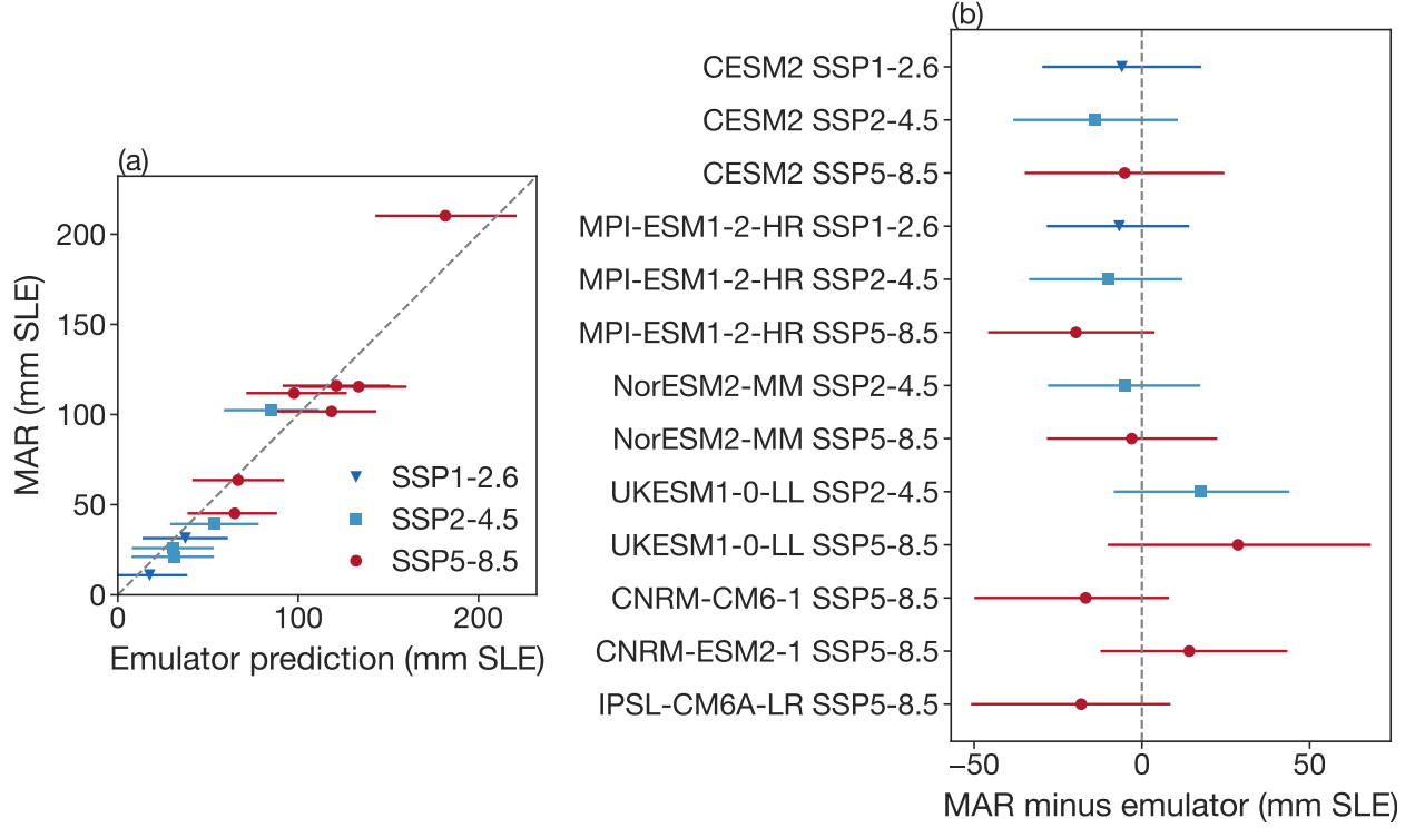
Figure S7: Leave-one-GCM-out test of the Greenland SMB emulator. Each GCM is withheld in turn, and its SSP runs are predicted by the emulator fitted to the other six GCMs, driven by the withheld GCM’s GMST and anchored to its own 1995–2005 mean. (a) Cumulative SMB contribution over 2015–2100 relative to the 1995–2005 rate, MAR against the emulator. Horizontal bars show the 90% predictive range, which includes the spread of the six GCMs, the coefficient uncertainty, autoregressive weather noise, and the weather noise of the 1995–2005 anchor. The dashed line is the 1:1 line. (b) MAR minus the emulator median for each withheld run, with the same 90% range. Positive values mean that the emulator underpredicts the contribution to sea-level rise.
