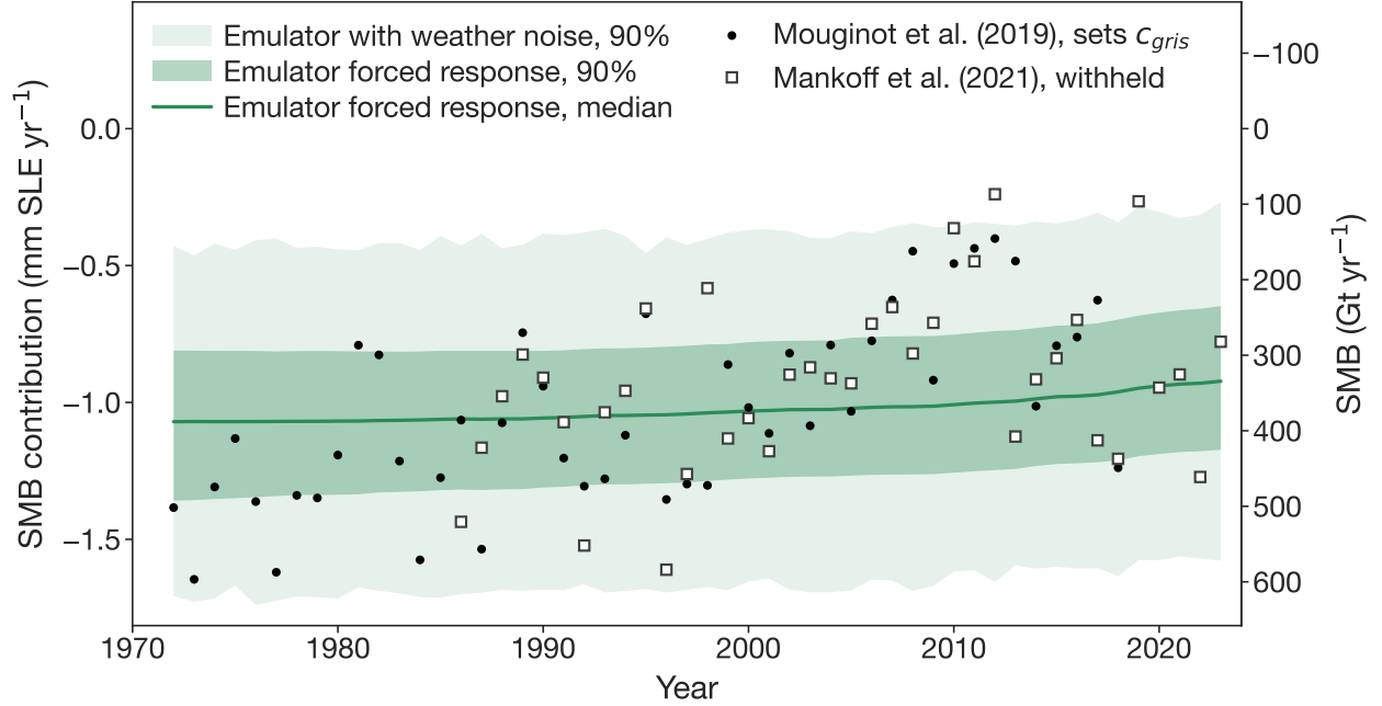
Figure S9: Greenland SMB emulator driven by observed GMST. The emulator’s forced response (dark band, 90% range, and median), driven by the Berkeley Earth GMST anomaly ( Rohde and Hausfather, 2020 ) with the 11-year centered mean used in training, is compared with the Mouginit et al. (2019) SMB, whose 1995–2005 mean anchors the emulator in this comparison, and the withheld Mankoff et al. (2021) SMB. The forced-response range includes the GCM, the coefficients, and the uncertainty of that anchor. The drift state is not included. The light band adds autoregressive weather noise with the parameters fitted to each GCM. The centered mean for 2020–2024 uses the IPCC AR6 SSP2-4.5 GMST path ( Lee et al., 2021 ) for 2025–2029. The right axis gives the same SMB in Gt yr -1 .
