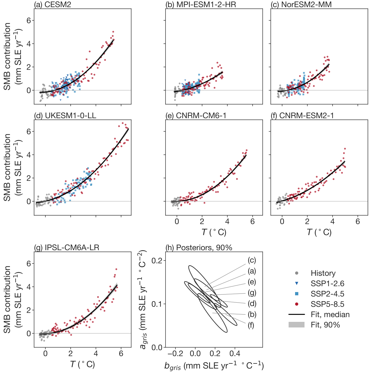
Figure S6: Greenland SMB emulator fits. (a–g) Annual SMB contribution of the contiguous Greenland ice sheet simulated by MARv3.12 driven by each of seven CMIP6 GCMs, relative to the 1995–2005 mean of that GCM’s history run, against the GCM’s own GMST anomaly T (11-year centered mean, relative to 1995–2005). Points are colored and shaped by experiment. Black curves show the posterior median of the fitted quadratic, including the fitted intercept, and gray bands its 90% credible interval. (h) 90% ellipse of the joint posterior of a_{gris} and b_{gris} for each GCM, labeled with the letter of its panel. All quantities are contributions to GMSL.
