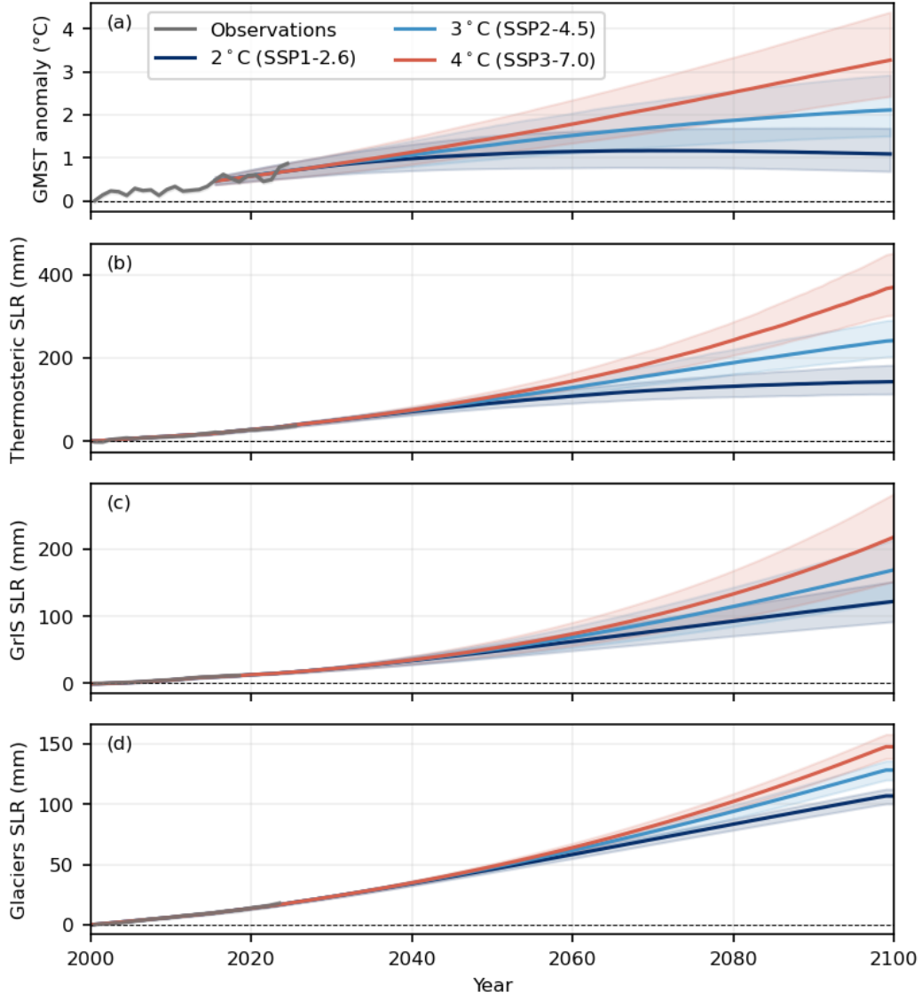
Figure 8: Component-level forecasts under three emissions scenarios. (a) Observed global mean surface temperature (GMST) anomaly (grey) relative to 2000, with SSP1-2.6, SSP2-4.5, and SSP3-7.0 projections (IPCC AR6) and their 90% CI (5–95th percentile, shaded). The SSP projections are labeled in the legend by their median 2100 anomaly relative to pre-industrial temperatures to provide both pre-industrial and 21st century baselines. (b) Thermosteric sea-level contribution: NOAA observations (grey) and forecast median with 90% CI from the full depth model driven by the corresponding GMST trajectory. (c) Greenland Ice Sheet (GrIS) contribution: observed cumulative mass balance (grey) and scenario forecasts from the discharge and SMB models. (d) Global glacier contribution: observations (grey) and scenario forecasts from the temperature-driven glacier model. Antarctic Peninsula and EAIS are excluded from this plot because their contributions are within the uncertainties of the components shown.
