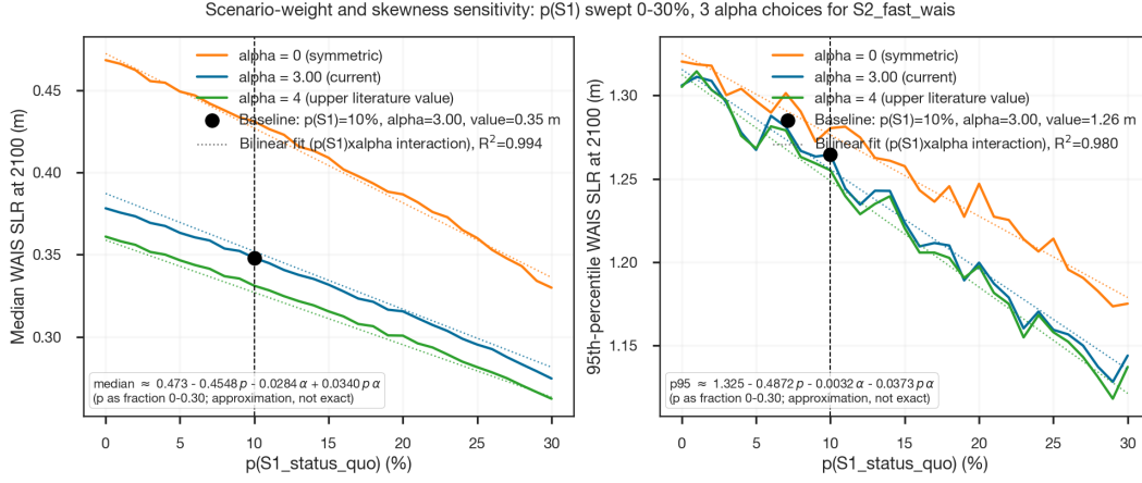
Figure S5: Scenario weight sensitivity. Median (left) and 95th-percentile (right) WAIS SLR at 2100 as a function of P(S1\_status\_quo) , swept from 0 to 30% ( P(S2\_fast\_wais) = 1 - P(S1) ). The marker indicates the baseline value ( P(S1) = 0.10 ). Both statistics vary only modestly across the swept range, confirming that within-scenario uncertainty dominates over the assigned scenario weight.
