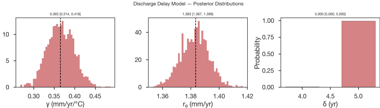
Figure S1: Greenland discharge delay model parameter posteriors. Marginal posteriors for the three parameters of the discharge delay model calibrated against Mouginot et al. (2019). (a) The sensitivity of discharge to cumulative delayed ocean thermal forcing, \gamma , and (b) the background discharge rate, r_0 . Both are shown as the exact marginal density, a mixture of normals over the candidate delays weighted by the Bayesian Information Criterion, rather than as a histogram of posterior draws. Dashed lines mark the posterior median and dotted lines the 5th and 95th percentiles. (c) The delay \delta is resolved only to integer years, so its posterior is the set of weights over the candidate delays, which place 99.5% of the weight on \delta = 5 yr. Panel titles give the median with the 90% credible interval.
