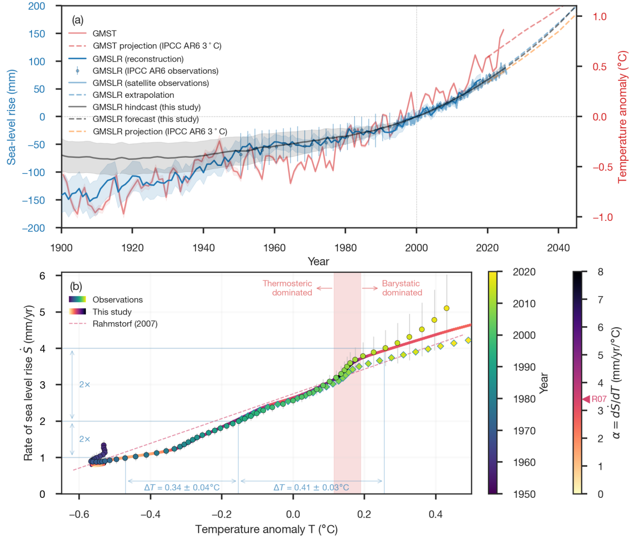
Figure 9: Observed global mean sea-level rise and global mean surface temperature. (a) GMSL reconstructions (blue line Frederikse et al. (2020); blue circles Fox-Kemper et al. (2021)) along with more recent NASA satellite altimetry (light blue; Beckley et al. (2017)) show sea-levels rising with warming. Hindcast results of this study (grey line with 90% CI shading) show good agreement back to 1950, the earliest year when GMSL reconstructions agree ( Fox-Kemper et al. , 2021). Different projection methods (dashed lines) show the divergence of IPCC AR6 projections and observed trends within a decade. GMST (red; ( Rohde and Hausfather , 2020)) is referenced to the right hand axis. (b) Rate of GMSL rise ( \dot{S} = dGMSL/dt ) versus GMST anomaly, T . Observed values are shown in circles ( Frederikse et al. , 2020) and diamonds ( Beckley et al. , 2017), colored by year, and the component model of this study is a line colored by instantaneous transient sensitivity \alpha = d\dot{S}/dT . The Rahmstorf (2007) semi-empirical model is shown in a color corresponding to its \alpha value ( Rahmstorf , 2007). The vertical red band indicates the shift in the primary contributor from ocean thermal expansion to changes in glacier ice and water storage (barystatic). The sinuous tail in the early observations is largely due to dam impoundment of water rather than a thermodynamic signal ( Frederikse et al. , 2020).
