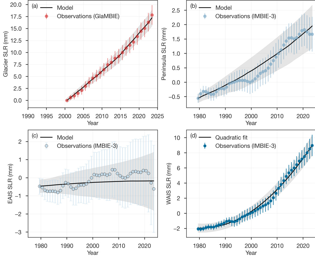
Figure 4: Per-component calibration fits. (a) Glaciers, (b) Antarctic Peninsula, and (c) EAIS observed mass balance (circles with \pm 2 standard deviation error bars) with the respective posterior median rate-temperature models (black lines) and 90% credible interval (gray shading). (d) WAIS mass balance is shown with the quadratic-in-time model (black line) and 90% credible interval (gray shading). Data are from The GlaMBIE Team et al. (2025) for glaciers and Otosaka et al. (2026) for the ice sheets.
