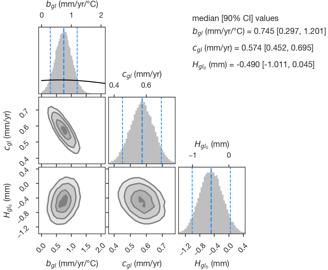
Figure 5: Glacier model posterior correlation structure. The joint posterior for the three parameters of the level-space glacier model ( b_{gl} , c_{gl} , H_{gl0} ) fitted to the GlaMBIE record. Diagonal panels show marginal posterior histograms, with dashed vertical lines marking the median and 90% credible interval. Off-diagonal panels show the joint posterior density, with contours denoting 1, 2, and 3 standard deviations. Only b_{gl} has an informative prior (black curve), centered on Rounce et al. (2023) and wide enough to be only weakly informative over the range the data support. The warming sensitivity b_{gl} and the baseline offset H_{gl0} are only weakly correlated because the temperature integral is anchored at the study’s baseline year (2000) rather than at the start of the temperature record, leaving H_{gl0} little leverage over the fitted trend; b_{gl} and the committed rate c_{gl} show the anti-correlation expected of a slope and intercept fit over a temperature record not centered on zero.
