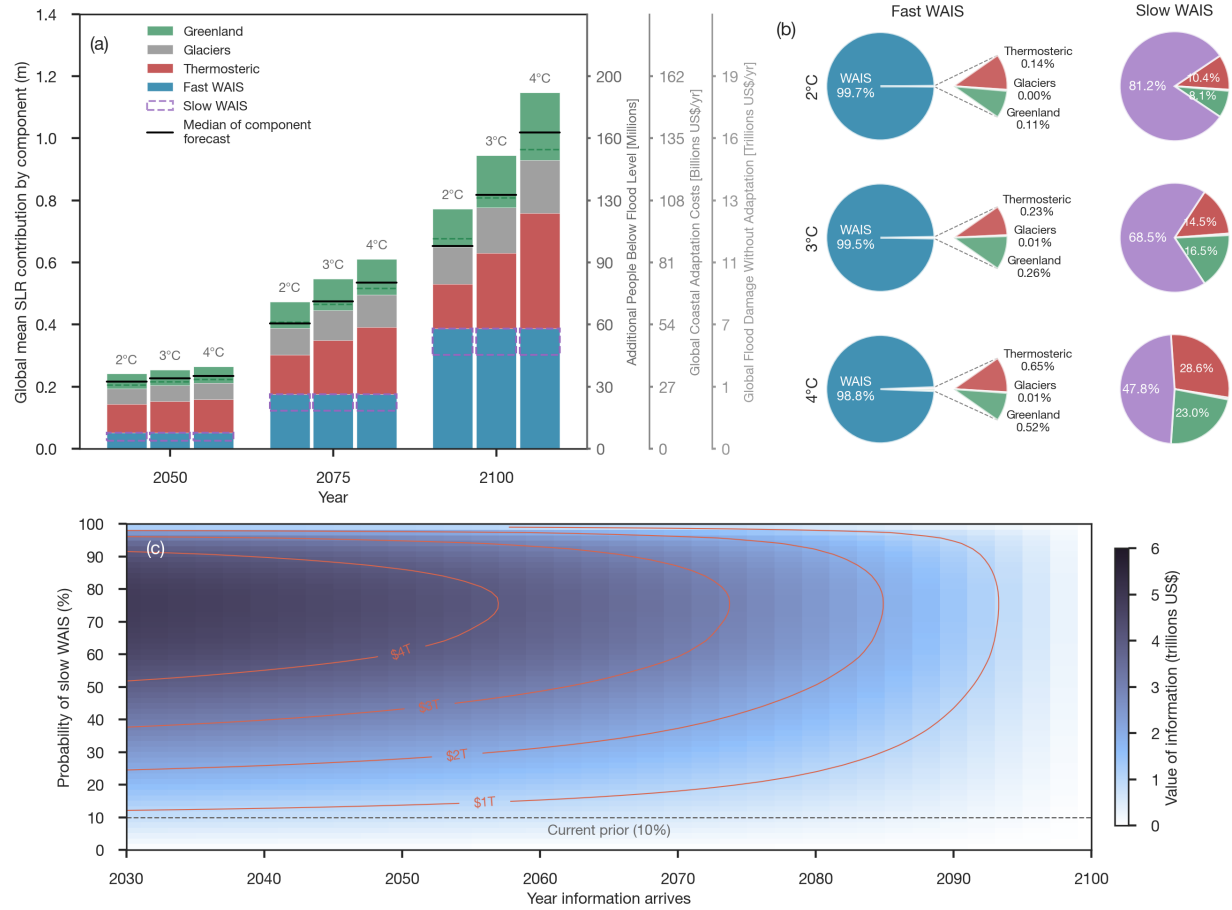
Figure 12: Component contributions, variance decomposition, and value of information. (a) 21st century mean GMSLR contribution by component and respective societal costs. Green dashed lines within Greenland bars partition discharge anomaly (below) from SMB anomaly (above). The purple box shows how much WAIS will contribute if it loses mass slowly while the rest of the blue bar shows the potential SLR from rapid ice loss. (b) Variance-fractions at 2100. WAIS accounts for approximately 99% of total forecast variance when rapid ice loss is possible. Fan breakouts show the non-WAIS contributions. If WAIS loses mass slowly, the variance distributions fundamentally shift (right column) (c) Financial value of resolving WAIS uncertainty as a function of when information arrives. Contours and colormap in trillions US$ based on coastal adaptation costs (Supplemental Material). The plot shows that information has more value if it arrives early enough to inform key decisions and if it provides sufficient confidence that WAIS will lose mass slowly, allowing planning around lower future sea levels.
