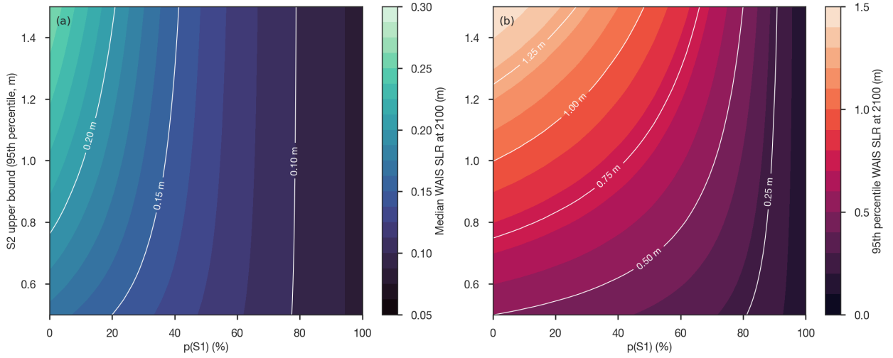
Figure 7: WAIS contribution to GMSL at 2100 as a function of the two mixture parameters. (a) Median and (b) 95th percentile of the S1/S2 mixture (relative to 2000) across the S1 probability, p(S1) , and the S2 upper bound (95th percentile of S2 at 2100).
