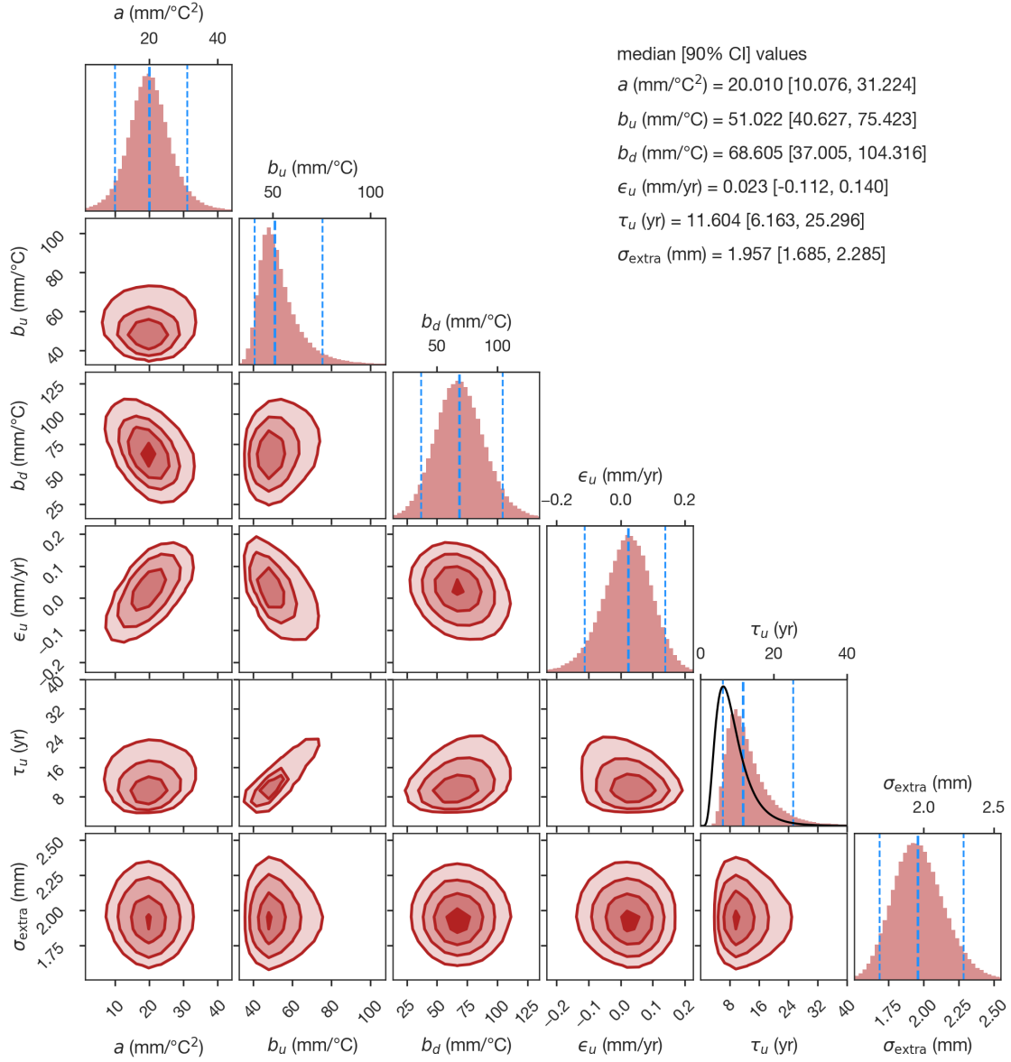
Figure 2: Two-layer thermosteric model posterior correlation structure. The joint posterior for the six parameters of the two-layer energy balance model fitted to NOAA 0–700 m and 0–2000 m thermosteric sea level data. Diagonal panels show marginal posterior histograms (red), with dashed vertical lines marking the median and 90% credible interval. Off-diagonal panels show the joint posterior density, with contours denoting 1, 2, and 3 standard deviations. Only \tau_u has an informative prior (black curve) while the other five parameters have flat, uninformative priors (not shown).
