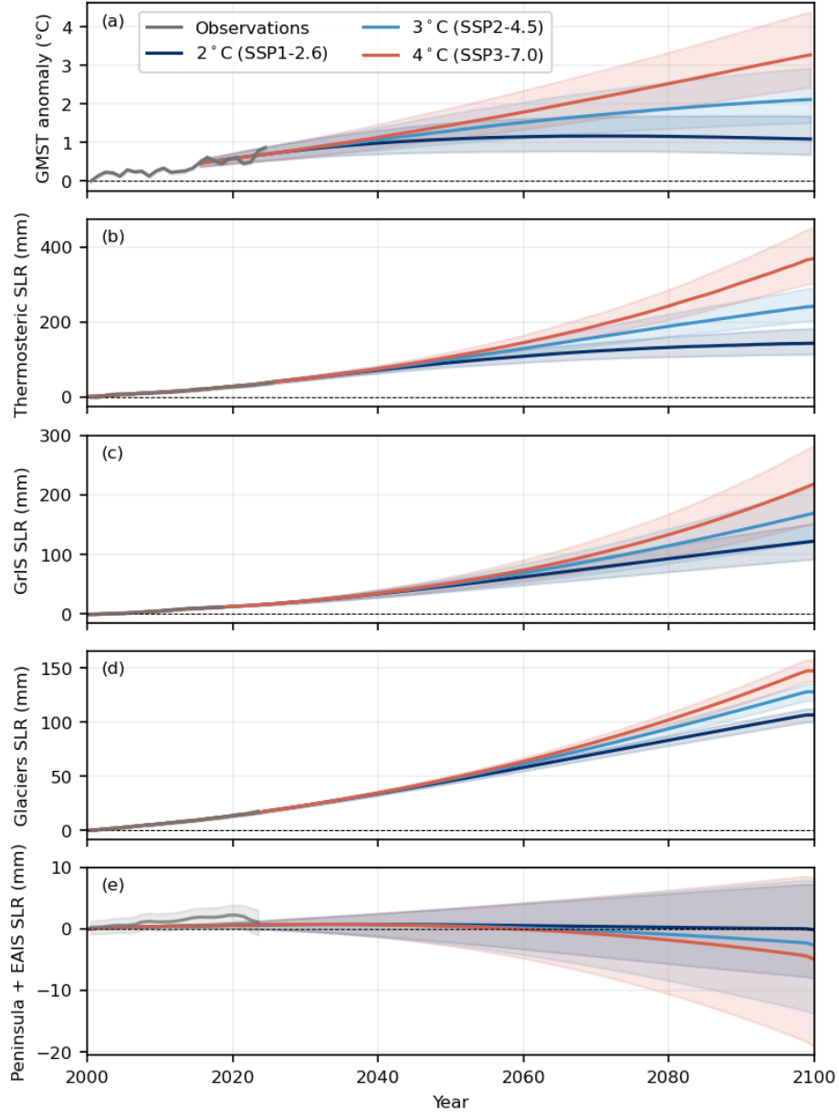
Figure 10: Component-level forecasts under three emissions scenarios. (a) Observed global mean surface temperature (GMST) anomaly (grey) relative to 2000, with SSP1-2.6, SSP2-4.5, and SSP3-7.0 projections (IPCC AR6) and their 90% CI (5–95th percentile, shaded). The SSP projections are labeled in the legend by their median 2100 anomaly relative to pre-industrial temperatures to provide both pre-industrial and 21st century base-lines. (b) Thermosteric sea-level contribution with observations (grey) and forecast median with 90% CI from the full depth model driven by the corresponding GMST trajectory. (c) Greenland Ice Sheet (GrIS), (d) glaciers, and (e) the sum of Antarctic Peninsula and EAIS following the same convention as in (b).
