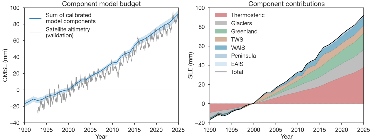
Figure 8: Budget closure: sum of model components versus observed GMSL. (a) Sum of components (blue) and NASA satellite altimetry (grey) with shaded band showing the 90% confidence intervals ( Beckley et al., 2017; Hamlington et al., 2020 ). (b) Stacked per-component contributions and their sum in black.
