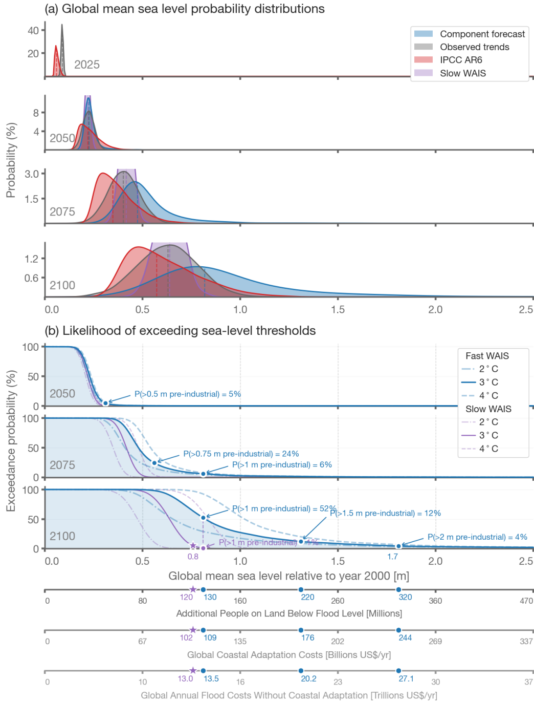
Figure 11: Global mean sea-level probabilities. (a) Probability distributions for different forecasting approaches and the IPCC AR6 projections. The ‘slow WAIS’ scenario (purple, clipped for figure clarity) assumes mass loss does not accelerate outside of the observed bounds (Scenario 1) while the component forecast (blue curve) allows for accelerated WAIS mass loss. Vertical dashed lines indicate the respective medians. (b) Probability of exceeding a given sea-level threshold for different warming trajectories including the WAIS scenario mixture model that allows for fast mass loss (blue) and the slow WAIS scenario (purple). Lower axes show estimates of the corresponding number of people currently living on land that will be below flood level ( Kulp and Strauss, 2019 ) and financial costs ( Tiggeloven et al., 2020; Jevrejeva et al., 2018 ) (Supplementary Material). Purple star indicates the 5% exceedance probability for the case that WAIS.
