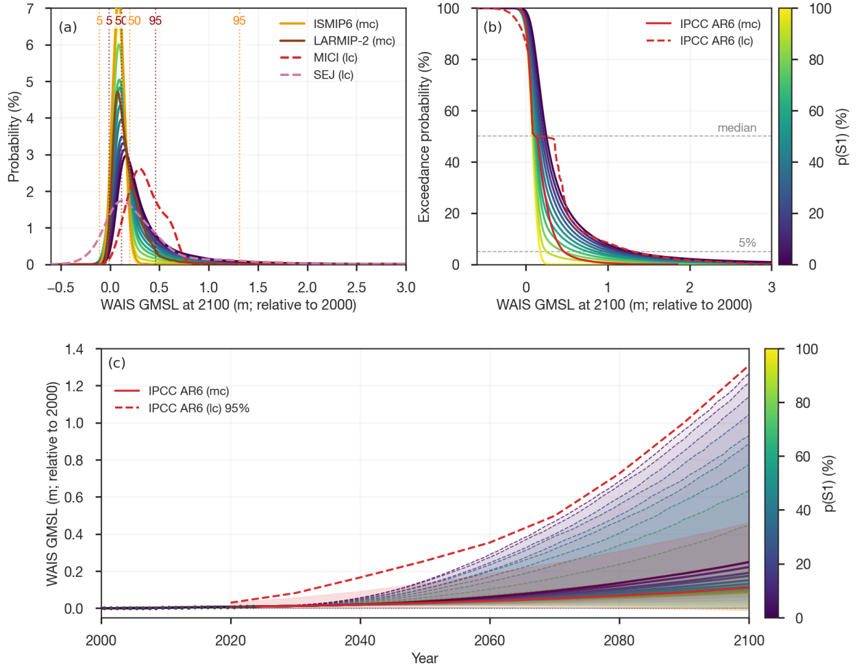
Figure 6: Sensitivity of the WAIS 2100 sea-level contribution to the S1/S2 scenario-mixture weight. (a) Probability density of the WAIS contribution to GMSL at 2100 (relative to 2000) for an 11-member sweep of the mixture weight p(S1) from 0% (Scenario 2) to 100% (Scenario 1), colored by weight (colorbar in b ). Also shown are the constituent IPCC AR6 total-Antarctic-Ice-Sheet workflow ensembles underlying the medium-confidence (mc, ISMIP6 emulator (Edwards et al., 2021) and LARMIP-2 ensemble (Levermann et al., 2020)) and low-confidence (lc) assessments. The low-confidence assessments are identified as Marine Ice Cliff Instability (MICI) (DeConto and Pollard, 2016) and structured expert judgement (SEJ) (Bamber et al., 2019). Dotted vertical lines mark the 5th, 50th, and 95th percentiles of the medium- (red) and low- (orange) confidence AR6 p-boxes. (b) Corresponding exceedance probability curves for the same p(S1) sweep, with the IPCC AR6 medium for 3 °C (SSP2-4.5; red solid line) and low-confidence SSP5-8.5 (red dashed line) exceedance curves for the Antarctic Ice Sheet overlaid for reference. (c) Time-series for the p(S1) sweep and the IPCC AR6 medium SSP2-4.5 (red solid line with 90% CI shading) and low-confidence SSP5-8.5 95th percentile (red dashed line). The thin dashed lines show the 95th percentile for the correspondingly colored p(S1) .
