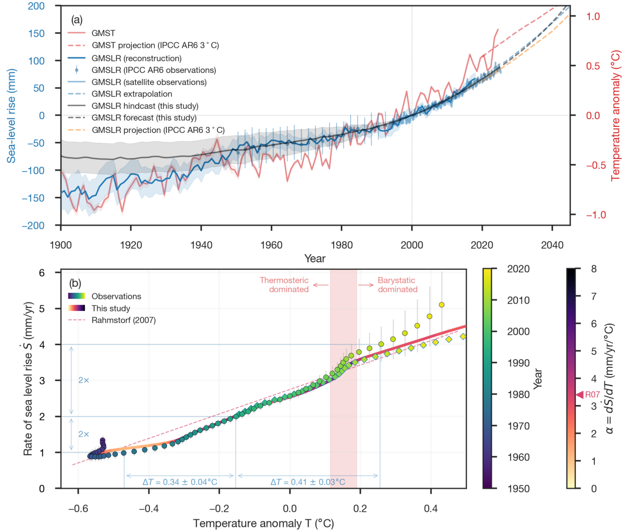
Figure 8: Observed global mean sea-level rises with global mean surface temperature. (a) GMSLR from reconstructions and tide-gauge records (blue line Frederikse et al. , 2020; blue circles Fox-Kemper et al. , 2021) along with more recent NASA satellite altimetry (light blue; Beckley et al. , 2017) show sea-levels rising with warming. Hindcast results of this study (grey line with 90% CI shading) show good agreement back to 1950, the earliest year when GMSLR reconstructions agree ( Fox-Kemper et al. , 2021). Different projection methods (dashed lines) show the divergence of IPCC AR6 projections and observed trends within a decade. GMST (red; Rohde and Hausfather , 2020) is referenced to the right hand axis. (b) Rate of GMSLR ( \dot{S} = d\text{GMSLR}/dt ) versus GMST anomaly, T . Observed values are shown in circles ( Frederikse et al. , 2020) and diamonds ( Beckley et al. , 2017), colored by year, and the component model of this study is a line colored by instantaneous transient sensitivity \alpha = d\dot{S}/dT . The Rahmstorf (2007) semi-empirical model is shown in a color corresponding to its \alpha value ( Rahmstorf , 2007). The vertical red band indicates the shift in the primary contributor from ocean thermal expansion to changes in glacier ice and water storage (barystatic). The sinuous tail in the early observations is largely due to dam impoundment of water rather than a thermodynamic signal ( Frederikse et al. , 2020).
