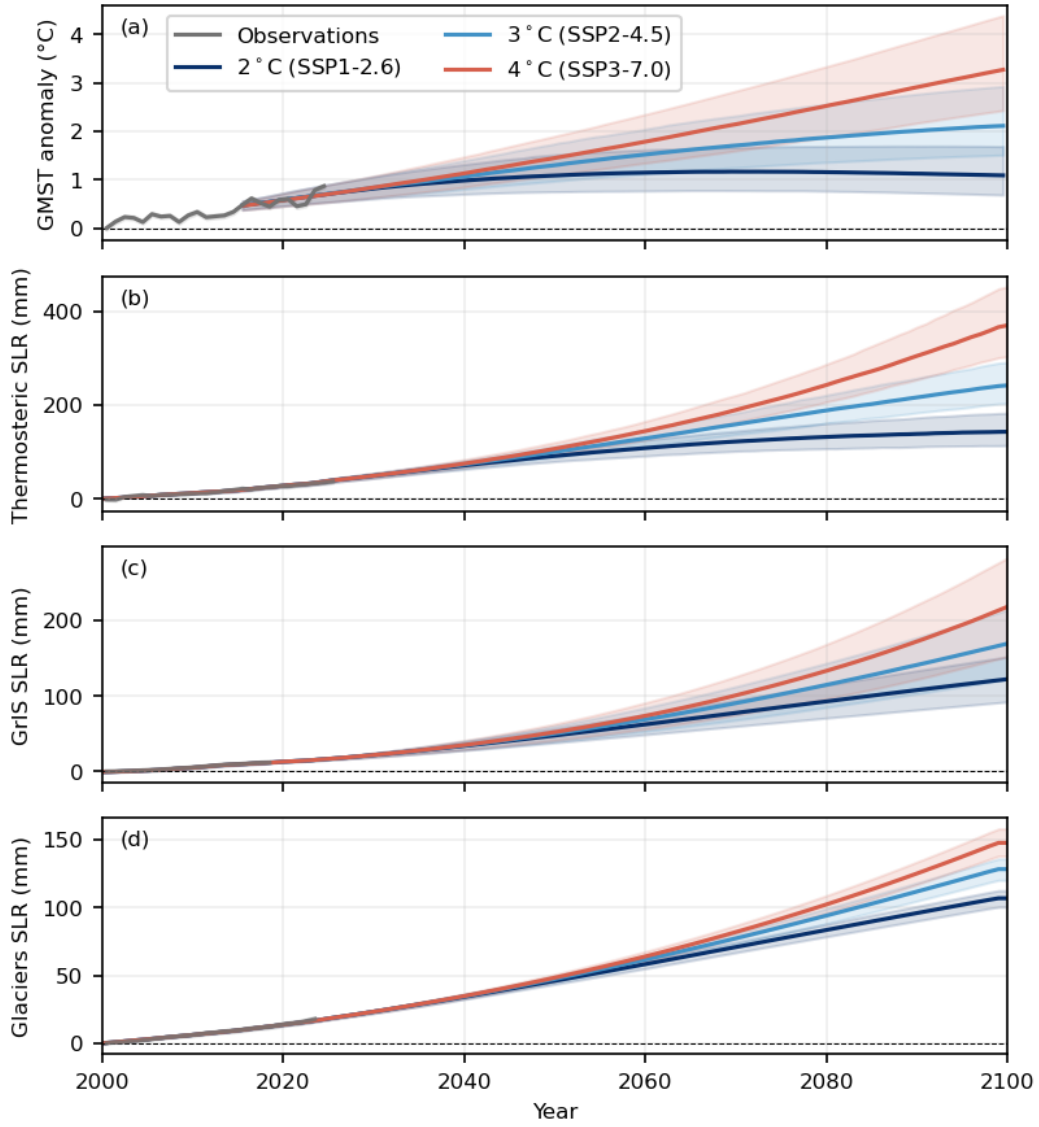
Figure 9: Component-level forecasts under three emissions scenarios. (a) Observed global mean surface temperature (GMST) anomaly (Berkeley Earth, grey) relative to 2000, with SSP1-2.6, SSP2-4.5, and SSP3-7.0 projections (IPCC AR6) and their 90% CI (5–95th percentile, shaded). The SSP projections are labeled in the legend by their median 2100 anomaly relative to pre-industrial temperatures to provide both pre-industrial and 21st century baselines. (b) Thermosteric sea-level contribution: NOAA observations (grey) and forecast median with 90% CI from the full depth model driven by the corresponding GMST trajectory. (c) Greenland Ice Sheet (GrIS) contribution: observed cumulative mass balance (grey) and scenario forecasts from the discharge and SMB models. (d) Global glacier contribution: observations (grey) and scenario forecasts from the temperature-driven glacier model.
