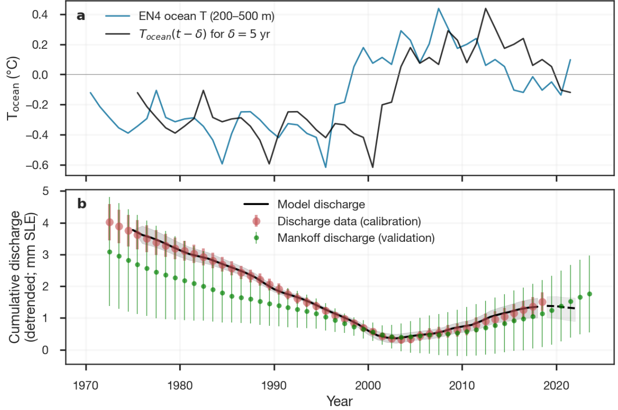
Figure 2: Greenland discharge delay model fit. (a) EN4 subsurface ocean temperature (200–500 m, annual) and the delayed signal T_{ocean}(t - \delta) with \delta = 5 yr. (b) Detrended cumulative Greenland ice discharge showing model fit (black) with 90% posterior CI, compared with the calibration (Mouginot et al. , 2019) and validation data (Mankoff et al. , 2021) in red and green, respectively.
