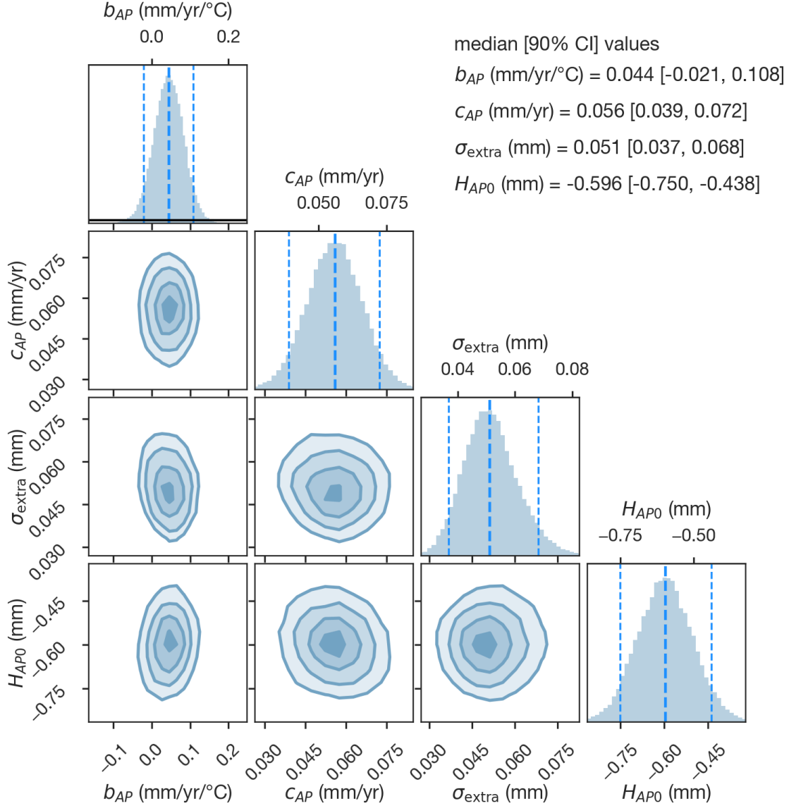
Figure S4: Antarctic Peninsula model posterior correlation structure. The joint posterior for the four parameters of the Peninsula model, the warming sensitivity b_{AP} , the committed rate c_{AP} , the model-inadequacy term \sigma_{\text{extra}} , and the baseline offset H_{AP0} , fitted to the IMBIE-3 Peninsula record ( Otosaka et al. , 2026) with the full covariance of the cumulative record in the likelihood. Diagonal panels show marginal posterior histograms, with dashed vertical lines marking the median and the 5th and 95th percentiles. Off-diagonal panels show the joint posterior density, with contours denoting 1, 2, and 3 standard deviations. Posterior medians are b_{AP} = 0.044 \text{ mm yr}^{-1} \text{ }^{\circ}\text{C}^{-1} [-0.021, 0.108], c_{AP} = 0.056 \text{ mm yr}^{-1} [0.039, 0.072], \sigma_{\text{extra}} = 0.051 \text{ mm} [0.037, 0.068], and H_{AP0} = -0.596 \text{ mm} [-0.750, -0.438], where brackets give 90% credible intervals. The prior on b_{AP} (black curve) is flat over the range the data support. The credible interval on b_{AP} spans zero, so the record does not resolve the sign of the temperature sensitivity, while the committed rate c_{AP} is well separated from zero. The posterior for \sigma_{\text{extra}} is likewise well separated from zero, confirming that the IMBIE-3 Peninsula record carries annual scatter beyond its reported uncertainty. All four parameters are close to mutually independent, the near-circular off-diagonal contours showing that the excess-noise term absorbs scatter without trading off against the fitted rate-temperature relationship.
