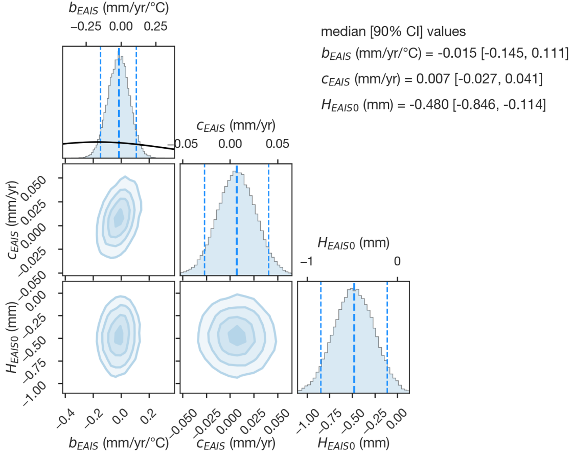
Figure S5: EAIS model posterior correlation structure. The joint posterior for the three parameters of the East Antarctic model, the warming sensitivity b_{EAIS} , the committed rate c_{EAIS} , and the baseline offset H_{EAIS0} , fitted to the IMBIE-3 East Antarctic record (Otosaka et al. , 2026) with the full covariance of the cumulative record in the likelihood. Diagonal panels show marginal posterior histograms, with dashed vertical lines marking the median and the 5th and 95th percentiles. Off-diagonal panels show the joint posterior density, with contours denoting 1, 2, and 3 standard deviations. Posterior medians are b_{EAIS} = -0.015 \text{ mm yr}^{-1} \text{ } ^\circ\text{C}^{-1} [-0.145, 0.111], c_{EAIS} = 0.007 \text{ mm yr}^{-1} [-0.027, 0.041], and H_{EAIS0} = -0.480 \text{ mm} [-0.846, -0.114], where brackets give 90% credible intervals. Only b_{EAIS} carries an informative prior (black curve), which is wide enough that the posterior is set by the data. Both the sensitivity and the committed rate have credible intervals spanning zero, consistent with an ice sheet close to balance over the IMBIE-3 record, which is why this fit serves as a diagnostic and the projection instead adopts the literature surface-mass-balance sensitivity C_T = 60 \pm 20 \text{ Gt yr}^{-1} \text{ } ^\circ\text{C}^{-1} (Frieler et al. , 2015; Ligtenberg et al. , 2013). The posterior is correspondingly uninformative in its correlation structure as well, with b_{EAIS} and c_{EAIS} weakly positively correlated and H_{EAIS0} nearly independent of both.
