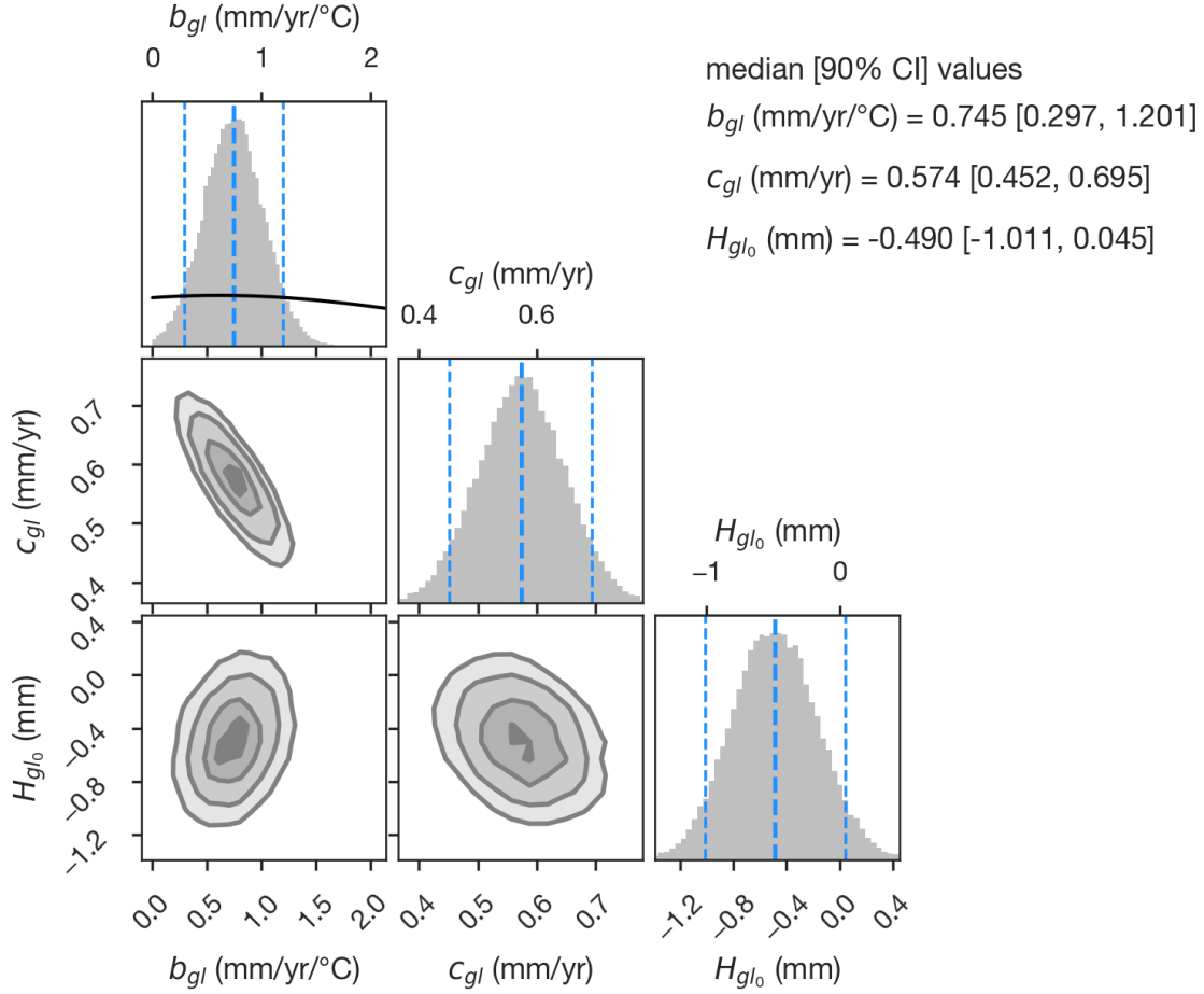
Figure S3: Glacier model posterior correlation structure. The joint posterior for the three parameters of the glacier model, the warming sensitivity b_{gl} , the committed rate c_{gl} , and the baseline offset H_{gl_0} , fitted to the GlaMBIE record ( The GlaMBIE Team et al. , 2025) with the full covariance of the cumulative record in the likelihood. Diagonal panels show marginal posterior histograms, with dashed vertical lines marking the median and the 5th and 95th percentiles. Off-diagonal panels show the joint posterior density, with contours denoting 1, 2, and 3 standard deviations. Posterior medians are b_{gl} = 0.745 \text{ mm yr}^{-1} \text{ } ^\circ\text{C}^{-1} [0.297, 1.201], c_{gl} = 0.574 \text{ mm yr}^{-1} [0.452, 0.695], and H_{gl_0} = -0.490 \text{ mm} [-1.011, 0.045], where brackets give 90% credible intervals. Only b_{gl} carries an informative prior (black curve), centered on the sensitivity of Rounce et al. (2023) and wide enough that the posterior is set by the data. The slope and intercept of a common record, b_{gl} and c_{gl} , are strongly anti-correlated, whereas H_{gl_0} is only weakly correlated with either because the temperature integral is anchored at the year 2000 baseline rather than at the start of the temperature record.
