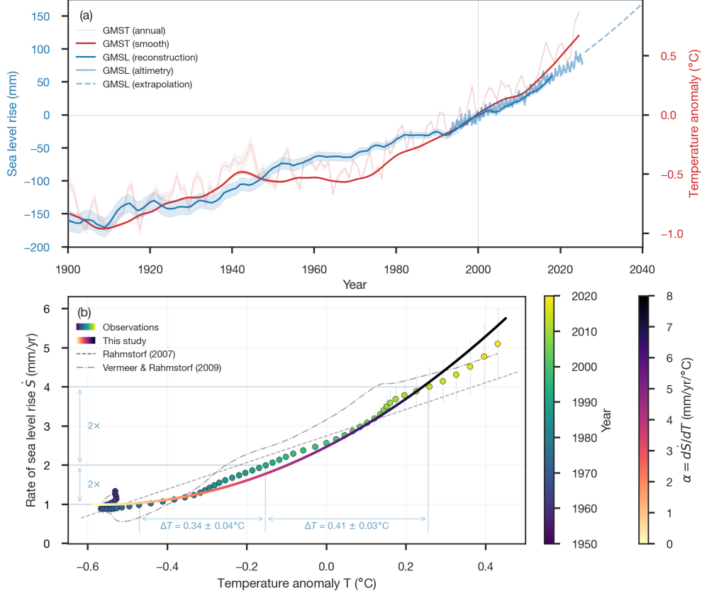
Figure 1: Observed global mean sea-level rise and its response to global mean surface temperature. (a) Observed GMSL (blue, 5-year smooth; Frederikse et al. [1]) and NASA satellite altimetry (light blue) since 1900, with the satellite-era quadratic extrapolation (dashed) and GMST (red, 15-year smooth; Berkeley Earth [2]) on the right axis. (b) GMSL rate versus GMST anomaly. Observations (circles, colored by year) and the Bayesian rate-and-state semi-empirical model of this study (colored by instantaneous transient sensitivity \alpha = d\dot{S}/dT ). Previous semi-empirical model results are shown as dashed [24] and dash-dot lines [25]. Horizontal and vertical lines mark the 1–2 and 2–4 mm yr -1 rate doublings that occurred during 1976–1992 (1959–1993, \pm 1\sigma ) and 1992–2013 (1992–2014, \pm 1\sigma ), respectively. The corresponding warming increments ( \Delta T ) show that the first doubling required slightly less warming ( 0.34 \pm 0.04 °C) than the second ( 0.41 \pm 0.03 °C).
