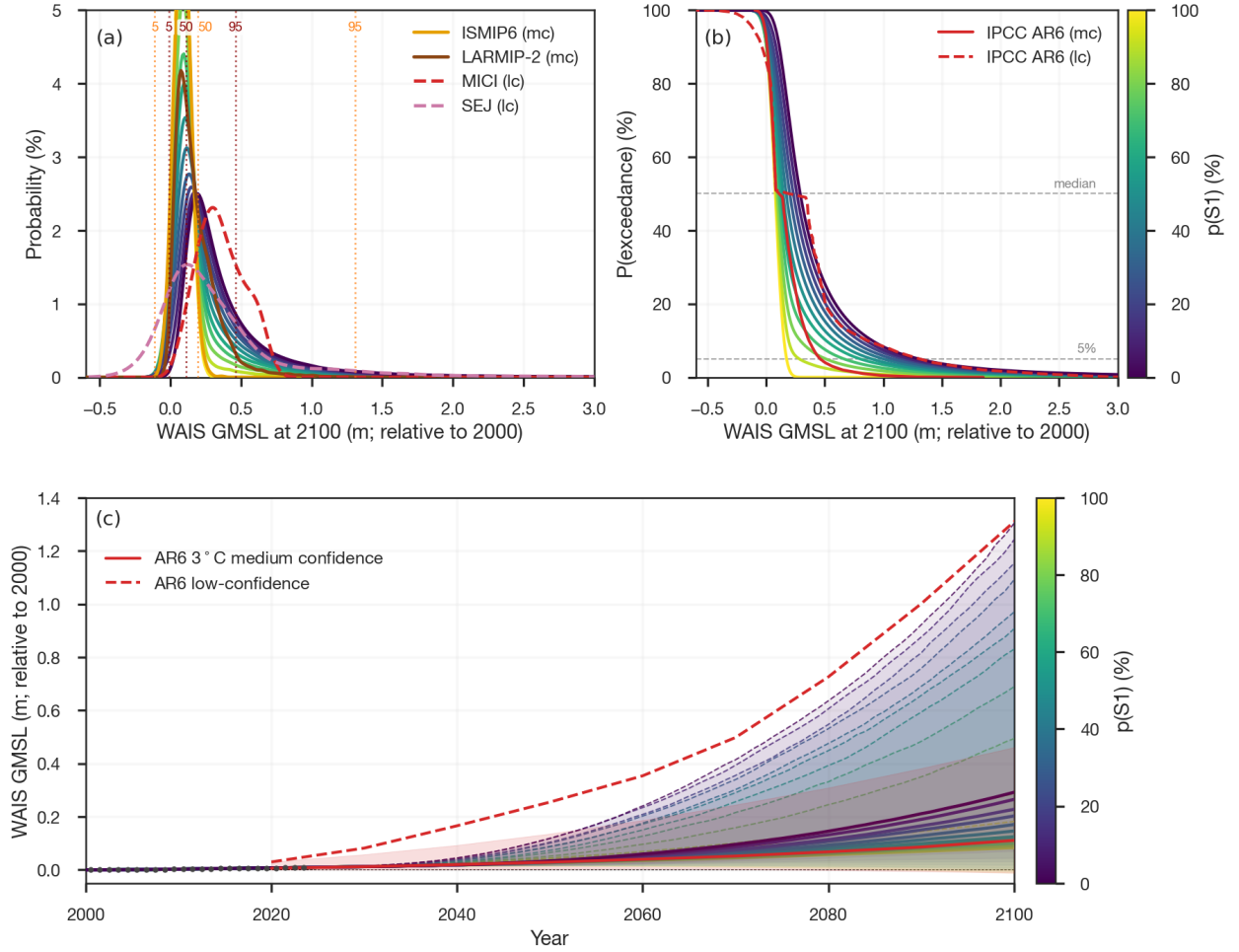
Figure 7: Sensitivity of the WAIS 2100 sea-level contribution to the S1/S2 scenario-mixture weight. (a) Probability density of the WAIS contribution to GMSL at 2100 (relative to 2000) for an 11-member sweep of the mixture weight p(S1) from 0% (pure MISI-driven ‘fast WAIS’, Scenario 2) to 100% (pure observed-trajectory continuation, Scenario 1), colored by weight (colorbar in b); the manuscript adopts p(S1) = 10\% . Also shown are the constituent IPCC AR6 total-Antarctic-Ice-Sheet workflow ensembles underlying the medium-confidence (ISMIP6 emulator ( Edwards et al. , 2021); LARMIP-2 ( Levermann et al. , 2020)) and low-confidence (MICI ( DeConto and Pollard , 2016); SEJ ( Bamber et al. , 2019)) assessments, with dotted vertical lines marking the 5th, 50th, and 95th percentiles of the medium- (red) and low- (orange) confidence AR6 p-boxes. (b) Corresponding exceedance-probability curves for the same p(S1) sweep, with the IPCC AR6 medium- (solid) and low-confidence (dashed) total-AIS exceedance curves overlaid for reference. Across the full range of p(S1) , the scenario mixture spans the medium- to low-confidence AR6 assessments.
