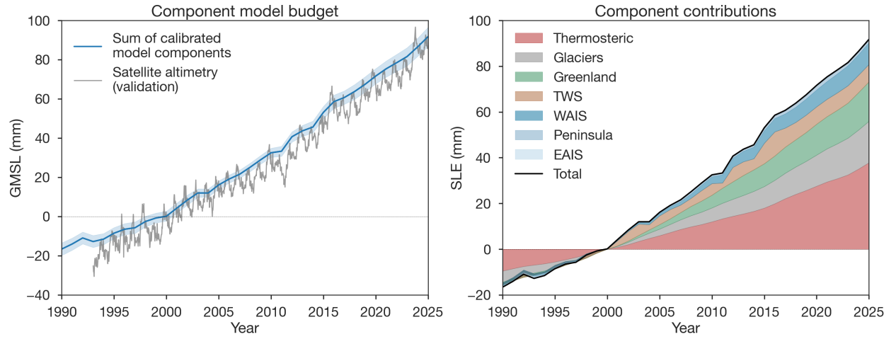
Figure 5: Budget closure: sum of model components versus observed GMSL. (a) Sum of components (blue) and NASA satellite altimetry (grey) with shaded band showing the 90% confidence intervals ( Beckley et al. , 2017; Hamlington et al. , 2020). (b) Stacked per-component contributions and their sum in black.
