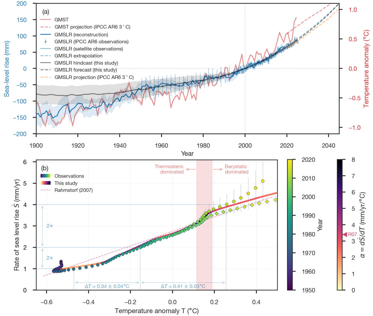
Figure 6: Observed global mean sea-level rise and global mean surface temperature. (a) GMSL reconstructions (blue line Frederikse et al. (2020); blue circles Fox-Kemper et al. (2021)) along with more recent NASA satellite altimetry (light blue; Beckley et al. (2017)) show sea-levels rising with warming. Hindcast results of this study (grey line with 90% CI shading) show good agreement back to 1950, the earliest year when GMSL reconstructions agree ( Fox-Kemper et al. , 2021). Different projection methods (dashed lines) show the divergence of IPCC AR6 projections and observed trends within a decade. GMST (red; ( Rohde and Hausfather , 2020)) is referenced to the right hand axis. (b) Rate of GMSL rise ( \dot{S} = dGMSL/dt ) versus GMST anomaly, T . Observed values are shown in circles ( Frederikse et al. , 2020) and diamonds ( Beckley et al. , 2017), colored by year, and the component model of this study is a line colored by instantaneous transient sensitivity \alpha = d\dot{S}/dT . The Rahmstorf (2007) semi-empirical model is shown in a color corresponding to its \alpha value ( Rahmstorf , 2007). The vertical red band indicates the shift in the primary contributor from ocean thermal expansion to changes in glacier ice and water storage (barystatic). The sinuous tail in the early observations is largely due to dam impoundment of water rather than a thermodynamic signal ( Frederikse et al. , 2020).
