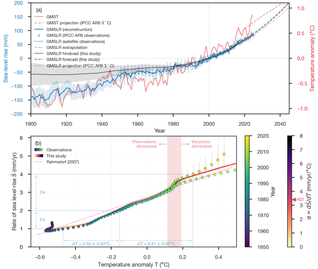
Figure 8: Observed global mean sea-level rise and global mean surface temperature. (a) GMSL reconstructions (blue line Frederikse et al. (2020); blue circles Fox-Kemper et al. (2021)) along with more recent NASA satellite altimetry (light blue; Beckley et al. (2017)) show sea-levels rising with warming. Hindcast results of this study (grey line with 90% CI shading) show good agreement back to 1950, the earliest year when GMSL reconstructions agree ( Fox-Kemper et al. , 2021). Different projection methods (dashed lines) show the divergence of IPCC AR6 projections and observed trends within a decade. GMST (red; ( Rohde and Hausfather , 2020)) is referenced to the right hand axis. (b) Rate of GMSL rise ( \dot{S} = dGMSL/dt ) versus GMST anomaly, T . Observed values are shown in circles ( Frederikse et al. , 2020) and diamonds ( Beckley et al. , 2017), colored by year, and the component model of this study is a line colored by instantaneous transient sensitivity \alpha = d\dot{S}/dT . The Rahmstorf (2007) semi-empirical model is shown in a color corresponding to its \alpha value ( Rahmstorf , 2007). The vertical red band indicates the shift in the primary contributor from ocean thermal expansion to changes in glacier ice and water storage (barystatic). The sinuous tail in the early observations is largely due to dam impoundment of water rather than a thermodynamic signal ( Frederikse et al. , 2020).
