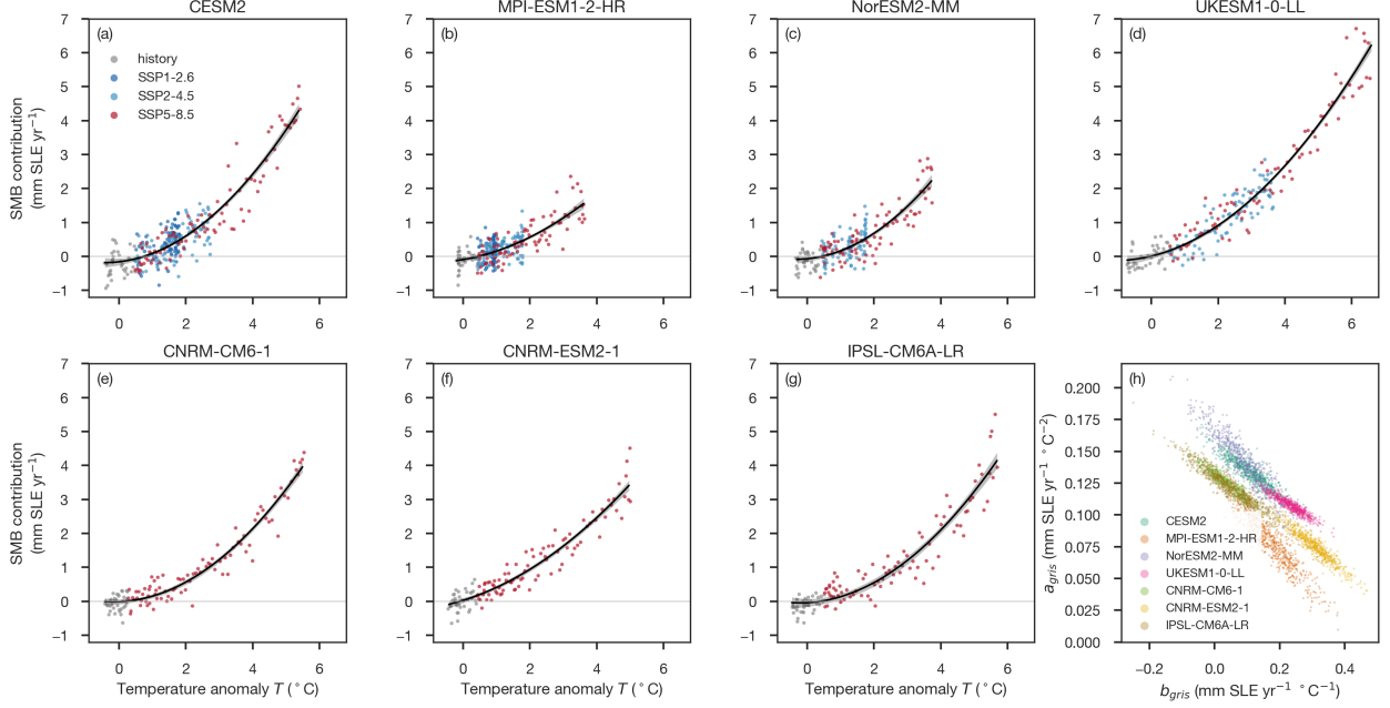
Figure S6: Greenland SMB emulator fits. (a–g) Annual SMB contribution of the contiguous Greenland ice sheet simulated by MARv3.12 driven by each of seven CMIP6 GCMs, relative to the 1995–2005 mean of that GCM’s history run, against the GCM’s own GMST anomaly T (11-year centered mean, relative to 1995–2005). Points are colored by experiment. Black curves show the posterior median of the fitted quadratic, including the fitted intercept, and gray bands its 90% credible interval. (h) Joint posterior of a_{gris} and b_{gris} for each GCM. All quantities are contributions to GMSL.
