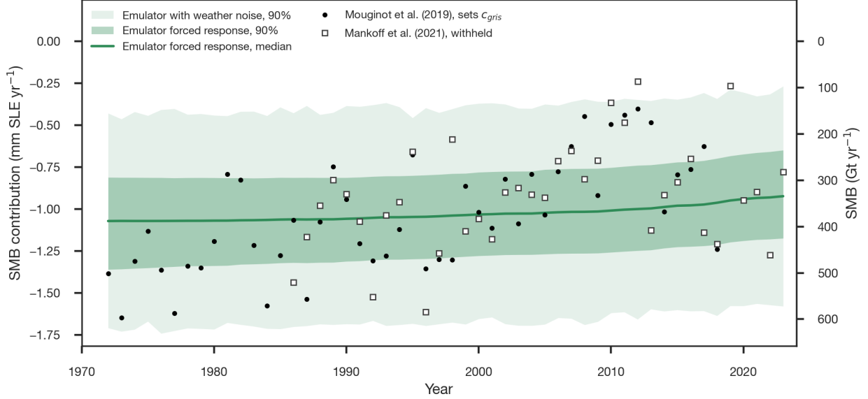
Figure S8: Greenland SMB emulator driven by observed GMST. The emulator’s forced response (dark band, 90% range, and median), driven by the Berkeley Earth GMST anomaly ( Rohde and Hausfather, 2020 ) with the 11-year centered mean used in training, is compared with the Mouginit et al. (2019) SMB, whose 1995–2005 mean anchors the emulator in this comparison, and the withheld Mankoff et al. (2021) SMB. The forced-response range includes the GCM, the coefficients, and the uncertainty of that anchor. The drift state is not included. The light band adds autoregressive weather noise with the parameters fitted to each GCM. The centered mean for 2020–2024 uses the IPCC AR6 SSP2-4.5 GMST path ( Lee et al., 2021 ) for 2025–2029. The right axis gives the same SMB in \text{Gt yr}^{-1} .
