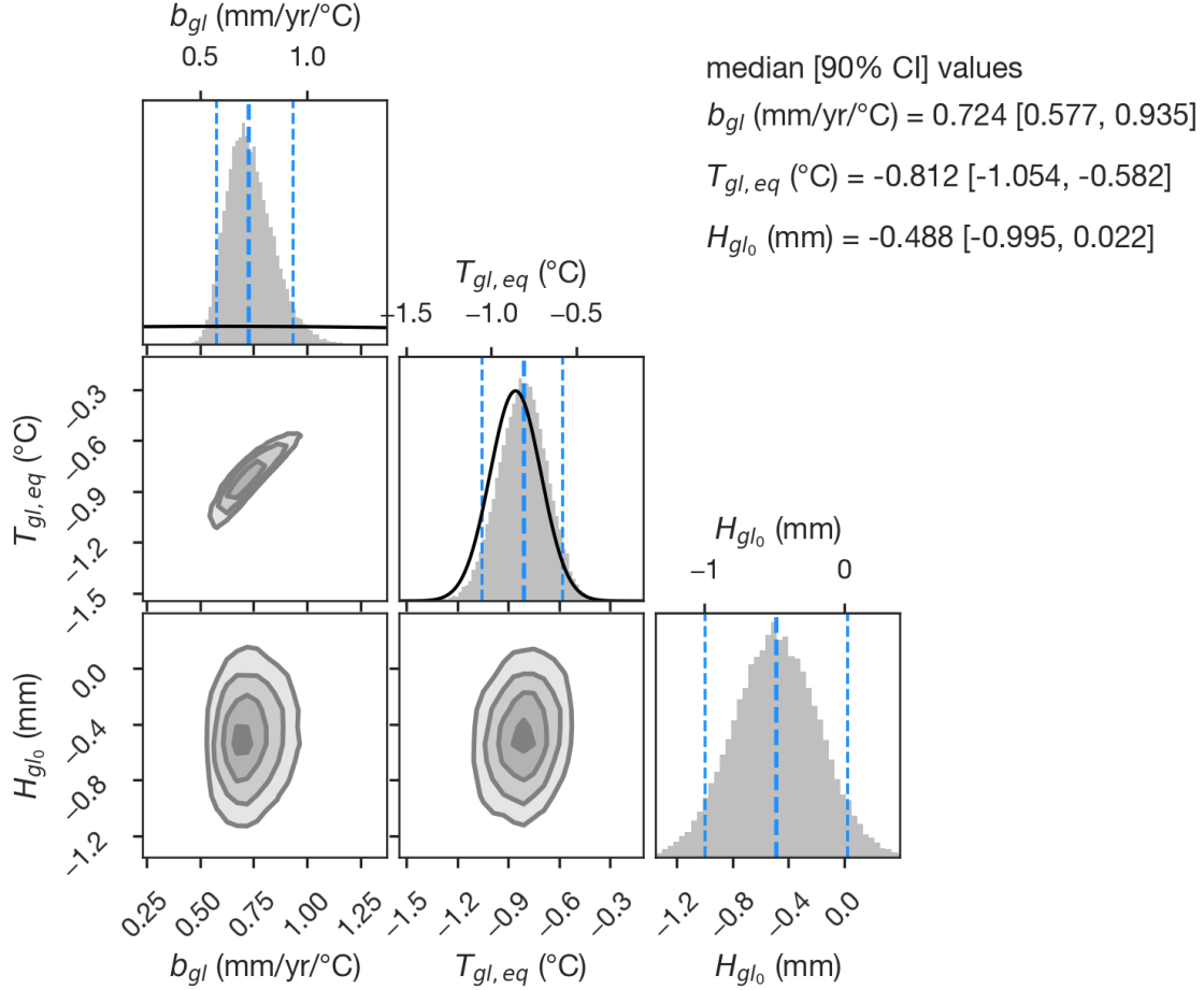
Figure S3: Glacier model posterior correlation structure. The joint posterior for the three free parameters of the glacier model ( b_{gl} , T_{gl,eq} , and H_{gl_0} ) fitted to the GlaMBIE record ( The GlaMBIE Team et al., 2025 ), with the full covariance of the cumulative record in the likelihood. Diagonal panels show marginal posterior histograms (gray), with dashed vertical lines marking the median and 90% credible interval. Off-diagonal panels show the joint posterior density, with contours denoting 1, 2, and 3 standard deviations. Black curves show the two informative priors, on b_{gl} , which is centered on the sensitivity of Rounce et al. (2023) and weakly informative, and on T_{gl,eq} , which is centered on the 1850–1879 mean GMST and fixes the committed rate c_{gl} = -b_{gl}T_{gl,eq} , while H_{gl_0} has a wide prior that is not shown.
