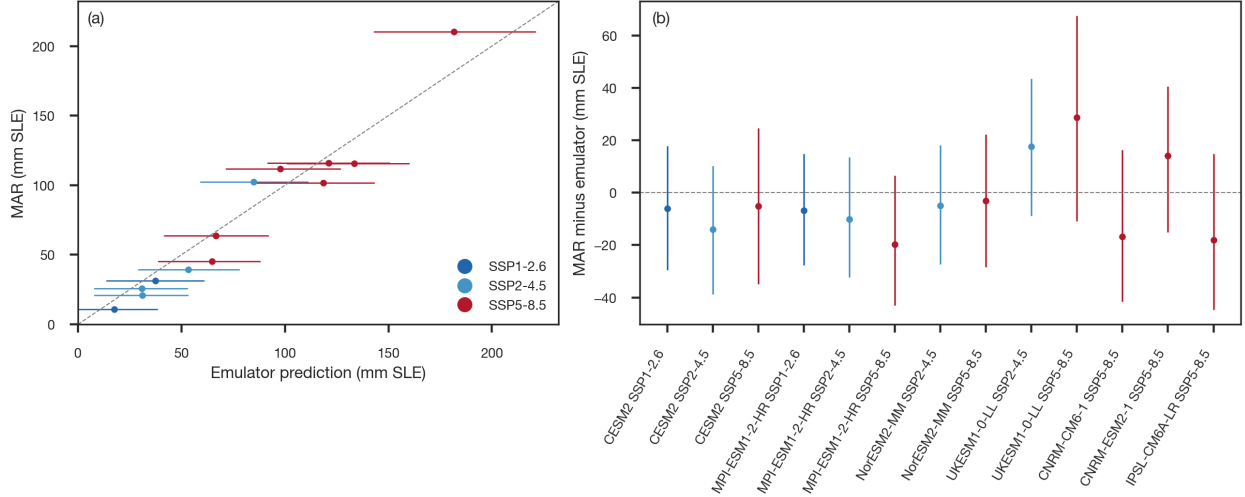
Figure S7: Leave-one-GCM-out test of the Greenland SMB emulator. Each GCM is withheld in turn, and its SSP runs are predicted by the emulator fitted to the other six GCMs, driven by the withheld GCM’s GMST and anchored to its own 1995–2005 mean. (a) Cumulative SMB contribution over 2015–2100 relative to the 1995–2005 rate, MAR against the emulator. Horizontal bars show the 90% predictive range, which includes the spread of the six GCMs, the coefficient uncertainty, autoregressive weather noise, and the weather noise of the 1995–2005 anchor. The dashed line is the 1:1 line. (b) MAR minus the emulator median for each withheld run, with the same 90% range. Positive values mean that the emulator underpredicts the contribution to sea-level rise.
