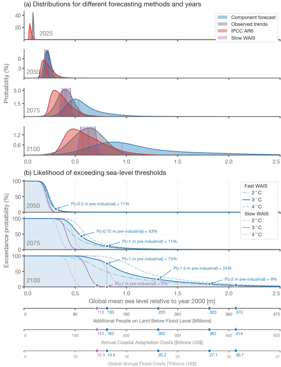
Figure 3: Distribution and exceedance probability of global mean sea-level projections. (a) Probability densities for the composite forecast of this study (blue), extrapolation of observations (grey; [2]), and IPCC AR6 projections (red; [12]). Vertical dashed lines indicate the respective medians. The purple band shows the 90% confidence interval for the case that WAIS does not experience a runaway acceleration, and sea level rise is due primarily to thermosteric, Greenland, and glaciers. We plot a purple band rather than distribution because the distribution is much tighter, and therefore taller, than the other distributions. (b) Probability of exceeding a given sea-level threshold for the 2°C (dash-dot), 3°C (solid), and 4°C (dashed) warming trajectories including instabilities in the West Antarctic Ice Sheet. Purple line shows the 3°C trajectory with a stable West Antarctic Ice Sheet. Lower axes show the corresponding number of additional people on land below flood level [7] and global annual flood costs [9], both assuming no additional coastal adaptation.
