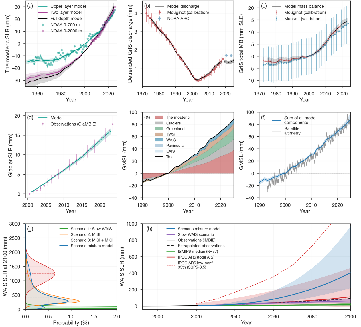
Figure 2: Model calibration, validation, and WAIS uncertainty. (a) Two-layer energy balance model fitted jointly to NOAA thermosteric sea level at 0–700 m (1955–2025) and 0–2000 m (2005–2025). (b) Greenland ice discharge modeled as a cumulative time-delay response to subsurface ocean warming ( \delta = 5 yr, rate-space R^2 = 0.79 ). Calibration data (Mouginitot et al. (2019) [33], filled circles) and withheld validation data (NOAA Arctic Report Card, diamonds) both fall within the 90% credible interval. (c) Global glacier contribution fitted to GlaMBIE consensus observations (2000–2023) using a linear temperature-driven model ( R^2 = 0.995 ). Grey band shows the 90% credible interval. (d,e) Budget closure: temperature-forced component hindcast (stacked) compared with NASA altimetry and reconstructions. The component sum closes the 2000–2025 budget to within 1%. (f) WAIS: IMBIE satellite observations (black) compared with the ISMIP6 ensemble median and interquartile range (green; [34]), our full scenario mixture (blue), the stable-WAIS scenario (purple), and IPCC AR6 total Antarctic projection (red).
