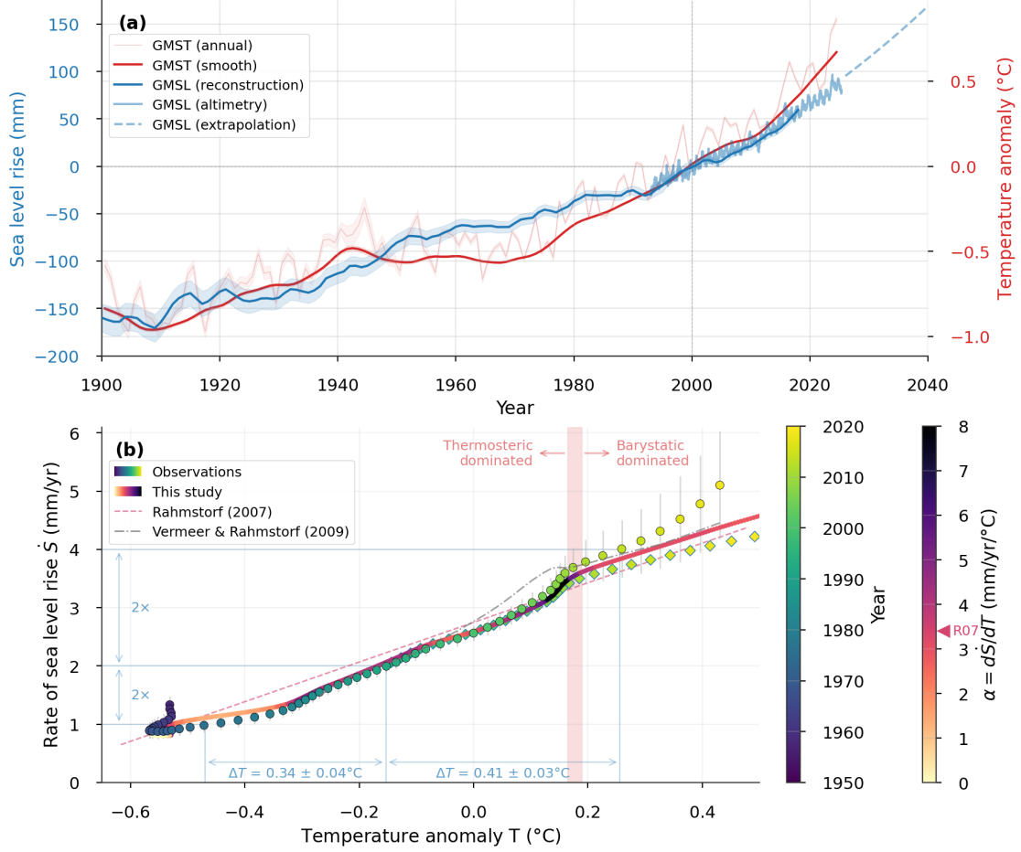
Figure 1: Observed global mean sea-level rise and its response to global mean surface temperature. (a) GMSL (blue, 5-year smooth; [1]) and NASA satellite altimetry (light blue; [4]), with the satellite-era quadratic extrapolation (dashed; [2]) and GMST (red, 15-year smooth [3]) on the right axis. (b) Rate of change in GMSL ( \dot{S} = dS/dt ) versus GMST anomaly, T . Observed values are shown in circles, colored by year, and the Bayesian rate-and-state semi-empirical model of this study are colored by instantaneous transient sensitivity \alpha = d\dot{S}/dT . Other semi-empirical model results are shown as dashed [5] and dash-dot lines [6]. Horizontal and vertical blue lines mark the 1–2 and 2–4 mm yr -1 rate doublings that occurred during 1976–1992 (1959–1993, \pm 1\sigma ) and 1992–2013 (1992–2014, \pm 1\sigma ), respectively. The corresponding warming increments ( \Delta T ) show that the first doubling required less warming ( 0.34 \pm 0.04 °C) than the second ( 0.41 \pm 0.03 °C). The vertical red band indicates the transition from thermosteric-dominated to barystatic-dominated sea-level rise (ocean mass change due to glaciers, ice sheets, and terrestrial water storage). The sinuous tail in the early observations is largely due to dam impoundment of water rather than a thermodynamic signal [1].
