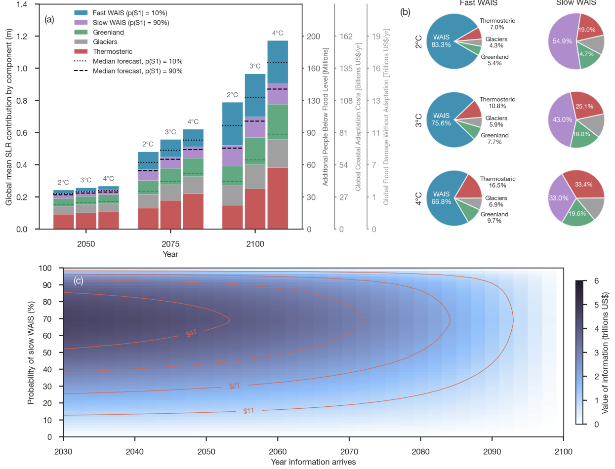
Figure 10: Component contributions, variance decomposition, and value of information. (a) 21st century mean GMSLR contribution by component and respective societal costs. The right-hand axes show the additional number of people on land below flood level ( Kulp and Strauss, 2019 ), global coastal adaptation costs ( Tiggeloven et al., 2020 ), and global flood damages without adaptation ( Jevrejeva et al., 2018 ) (Supplementary Material). Green dashed lines within Greenland bars partition discharge anomaly (below) from SMB anomaly (above). The purple box shows the WAIS contribution where slow mass loss is very likely, while the blue bar shows the additional potential SLR from rapid ice loss. (b) Shares of the 90% credible interval at 2100, taken as each component’s own interval width as a fraction of the summed widths. (c) Estimated financial value of resolving WAIS uncertainty as a function of when information arrives. Contours and colormap in trillions US$ based on coastal adaptation costs (Supplemental Material). The plot shows that information has more value if it arrives early enough to inform key decisions and if it provides sufficient confidence that WAIS will lose mass slowly, allowing planning around lower future sea levels.
