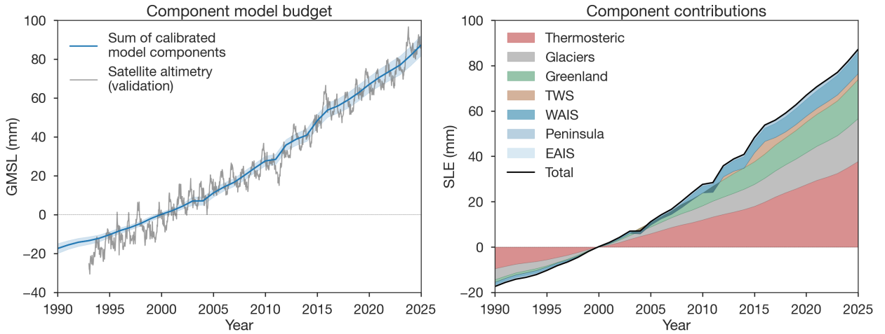
Figure 7: Budget closure: sum of model components versus observed GMSL. (a) Sum of components (blue) and NASA satellite altimetry (grey) with shaded band showing the 90% confidence intervals ( Beckley et al., 2017; Hamlington et al., 2020 ). (b) Stacked per-component contributions and their sum in black. Terrestrial water storage enters only from 2003, the start of the GRACE record from which it is derived.
