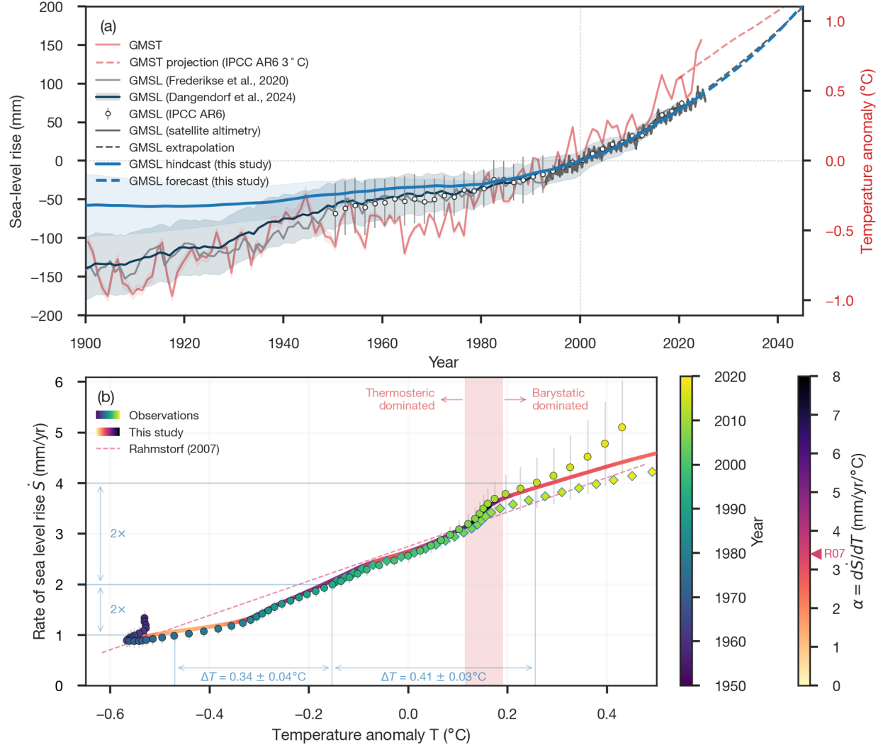
Figure 8: Observed global mean sea-level rise and global mean surface temperature. (a) GMSL reconstructions from Frederikse et al. (2020) (light grey) and Dangendorf et al. (2024) (navy, with 90% CI shading), the IPCC AR6 observational compilation ( Fox-Kemper et al. , 2021) (white circles with 90% CI bars), and NASA satellite altimetry ( Beckley et al. , 2017) (mid grey, with its quadratic extrapolation dashed) show sea level rising with warming. The hindcast and forecast of this study are shown in blue, solid and dashed respectively, with 90% CI shading. GMST (red; ( Rohde and Hausfather , 2020)) is referenced to the right hand axis. (b) Rate of GMSL rise ( \dot{S} = dGMSL/dt ) versus GMST anomaly, T . Observed values are shown in circles ( Frederikse et al. , 2020) and diamonds ( Beckley et al. , 2017), colored by year, and the component model of this study is a line colored by instantaneous transient sensitivity \alpha = d\dot{S}/dT . The Rahmstorf (2007) semi-empirical model is shown in a color corresponding to its \alpha value ( Rahmstorf , 2007). The vertical red band indicates the shift in the primary contributor from ocean thermal expansion to changes in glacier ice and water storage (barystatic). The sinuous tail in the early observations is largely due to dam impoundment of water rather than a thermodynamic signal ( Frederikse et al. , 2020).
