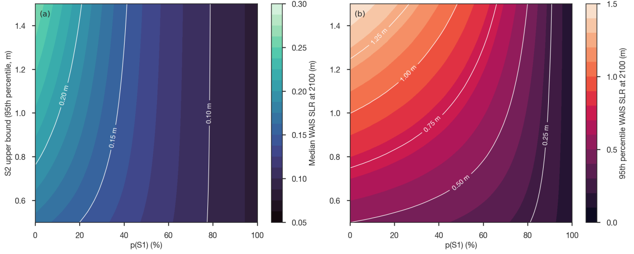
Figure 6: WAIS contribution to GMSL at 2100 as a function of the two mixture parameters. (a) Median and (b) 95th percentile of the S1/S2 mixture (relative to 2000) across the S1 probability, p(S1) , and the S2 upper bound (95th percentile of S2 at 2100).
