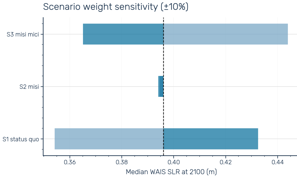
Figure 12: Scenario weight sensitivity. Tornado plot showing the effect of \pm 10 percentage-point perturbations to each scenario weight on the median WAIS SLR at 2100. Dark bars show the inner perturbation range; light bars extend to the full \pm 10\% range. The dashed vertical line indicates the baseline median (0.40 m). The mixture median is insensitive to weight perturbations, varying by less than 0.09 m across all perturbations—small relative to the 90% credible interval of the mixture distribution ( \sim 1.4 m).
