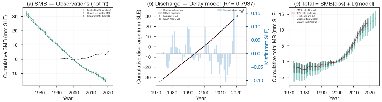
Figure 6: Greenland SMB, discharge, and total mass balance diagnostics. (a) Cumulative SMB from Mougnot (RACMO-derived), Mankoff, and GRACE – D implied SMB. SMB is used as observations, not fit to temperature. (b) Cumulative discharge from the delay model with 90% posterior CI, validated against Mougnot (calibration) and NOAA ARC (validation). (c) Total Greenland mass balance: SMB(obs) + D(model) compared with Mougnot (calibration) and Mankoff (validation) total mass balance records.
