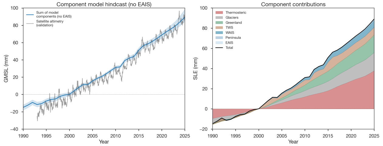
Figure 9: Budget closure: temperature-forced component hindcast versus observed GMSL. (a) Sum of components used for the budget-closure comparison (excluding EAIS; see text) against NASA satellite altimetry (grey); shaded band is the 5–95% Monte Carlo range. (b) Stacked per-component contributions to the hindcast, including EAIS; the black line is their sum. All values are relative to the year 2000 baseline.
