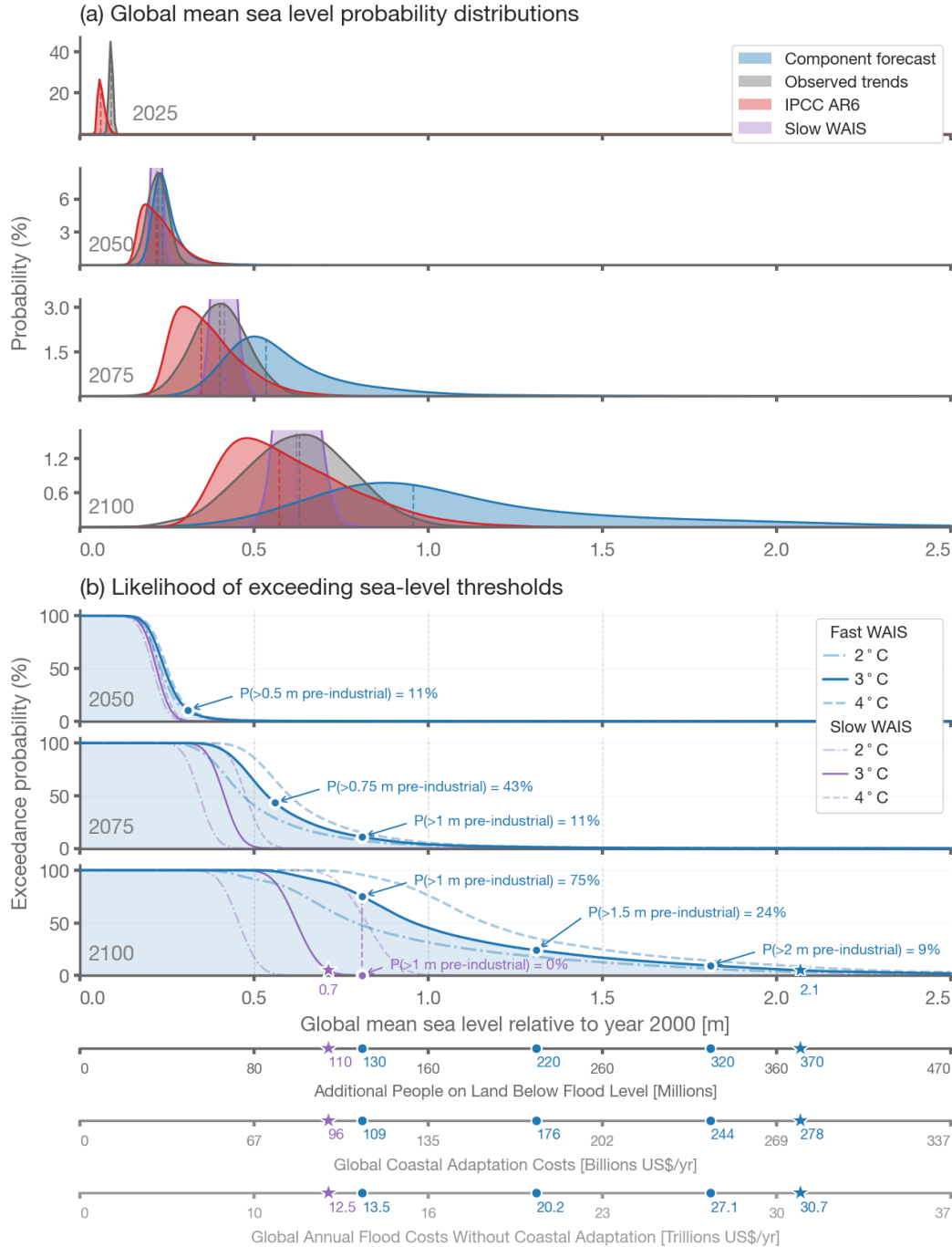
Figure 11: Global mean sea-level probabilities. (a) Probability distributions for different forecasting approaches and the IPCC projections. The ‘slow WAIS’ scenario (purple, clipped for clarity) assumes sustained mass loss at approximately modern rates (Scenario 1). Vertical dashed lines indicate the respective medians. (b) Probability of exceeding a given sea-level threshold for different warming trajectories including the WAIS scenario mixture model that allows for fast mass loss (blue) and the slow WAIS scenario (purple). Lower axes show estimates of the corresponding number of people currently living on land that will be below flood level (Kulp and Strauss, 2019) and financial costs (Tiggeloven et al., 2020; Jevrejeva et al., 2018) (Supplementary Material). Stars indicate the 5% exceedance probability.
