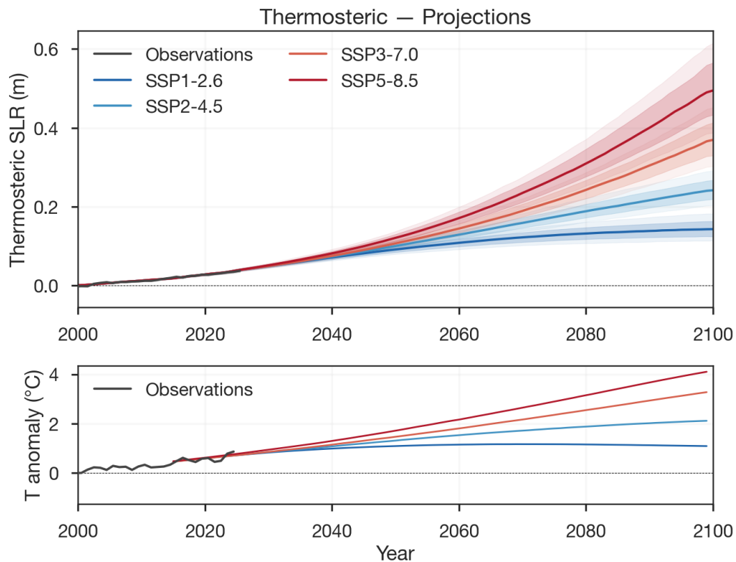
Figure 10: Thermosteric sea-level projections. Upper panel: median and 66%/90% credible intervals for the two-layer model under four SSP scenarios, with full-depth observations (black). Lower panel: GMST forcing trajectories (relative to year 2000) with Berkeley Earth observations.
