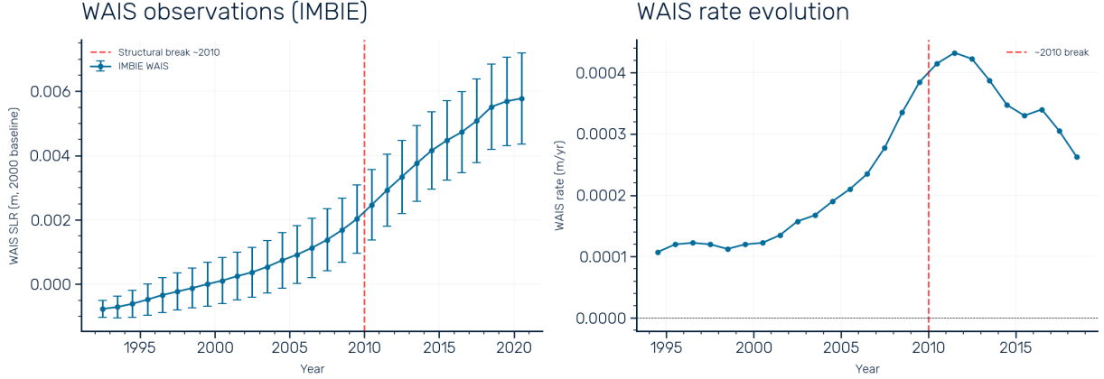
Figure S4: WAIS observational record. Left: cumulative WAIS sea-level contribution from IMBIE (1992–2020; Otosaka et al., 2023 ) with measurement uncertainties, relative to the year-2000 baseline. The structural break at \sim 2010 (red dashed line) separates a period of acceleration from apparent deceleration. Right: WAIS mass loss rate evolution, showing the rate increasing from \sim 0.15 \text{ mm yr}^{-1} in the early 1990s to a peak of \sim 0.44 \text{ mm yr}^{-1} around 2010–2012, followed by a decline that may reflect internal ocean variability in the Amundsen Sea ( Jenkins et al., 2018 ).
