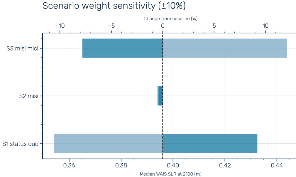
Figure S6: Scenario weight sensitivity. Tornado plot showing the effect of \pm 10 percentage-point perturbations to each scenario weight on the median WAIS SLR at 2100. Dark bars show the inner perturbation range; light bars extend to the full \pm 10\% range. The dashed vertical line indicates the baseline median (0.40 m). The mixture median is insensitive to weight perturbations, varying by less than 0.09 m across all perturbations—small relative to the 90% credible interval of the mixture distribution ( \sim 1.4 m).
