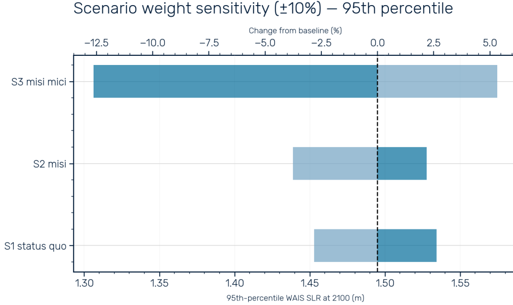
Figure S7: Scenario weight sensitivity—95th percentile. As in Fig. S6, but for the 95th percentile (5% exceedance) of the WAIS SLR distribution at 2100. The upper axis shows the percentage change from the baseline value ( \sim 1.5 m). The tail of the distribution is similarly insensitive to weight perturbations, with the largest shift ( \sim \pm 12\% from S3) remaining a small fraction of the total.
