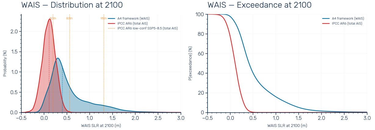
Figure S5: WAIS endpoint distributions and exceedance probabilities: A4 vs IPCC. Left: probability density at 2100 for the A4 WAIS framework (blue) compared with the IPCC AR6 total Antarctic projection (red). The A4 distribution is wider, with a higher median and a heavier right tail arising from the MISI skewness and rheology correction. Right: exceedance probability curves, showing that the A4 framework assigns substantially higher probability to exceeding any given threshold above \sim 0.1 m. The IPCC distribution assigns near-zero probability to outcomes exceeding 0.5 m, whereas the A4 framework assigns \sim 40\% probability to this threshold.
