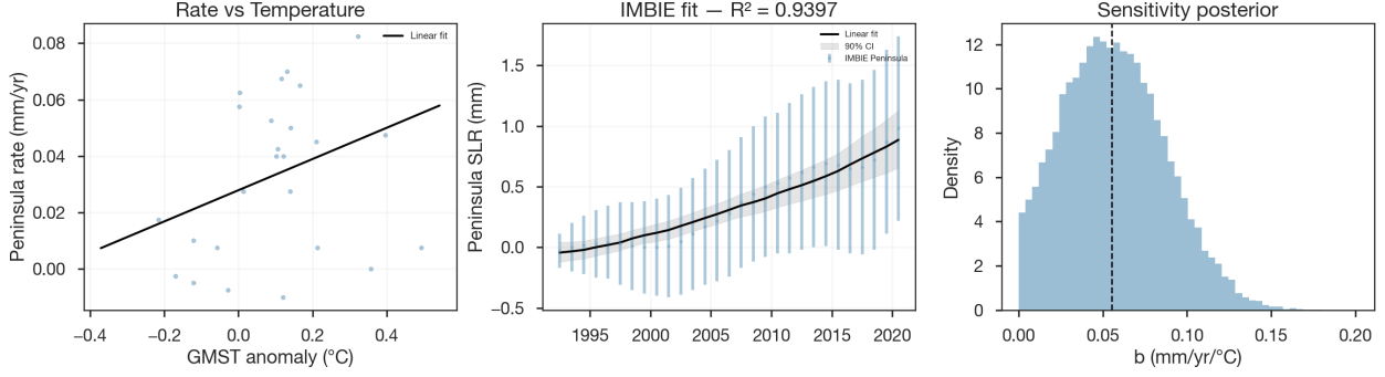
Figure S3: Peninsula model diagnostics. (a) Peninsula mass loss rate vs GMST anomaly with the fitted linear relationship. (b) Cumulative Peninsula SLR: IMBIE observations with the model fit and 90% credible interval; R^2 = 0.94 . (c) Posterior distribution for the temperature sensitivity b .
