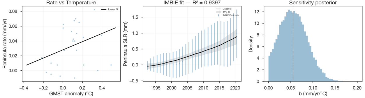
Figure S6: Peninsula model diagnostics. (a) Peninsula mass loss rate vs GMST anomaly with the fitted linear relationship. (b) Cumulative Peninsula SLR: IMBIE observations with the model fit and 90% credible interval; R^2 = 0.94 . (c) Posterior distribution for the temperature sensitivity b .
