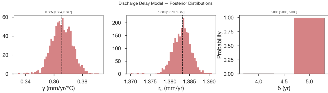
Figure S4: Greenland discharge model posteriors. Posterior distributions for the three parameters of the delay model: ocean thermal forcing sensitivity \gamma , background rate r_0 , and time delay \delta . The delay \delta is discrete (BIC-weighted mixture over \delta \in \{4, 5, 6, 7, 8\} yr); the remaining parameters are continuous.
