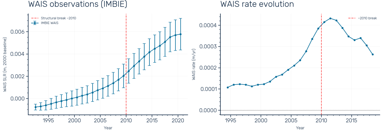
Figure S7: WAIS observational record. Left: cumulative WAIS sea-level contribution from IMBIE (1992–2020; Otosaka et al. , 2023) with measurement uncertainties, relative to the year-2000 baseline. The structural break at \sim 2010 (red dashed line) separates a period of acceleration from apparent deceleration. Right: WAIS mass loss rate evolution, showing the rate increasing from \sim 0.15 \text{ mm yr}^{-1} in the early 1990s to a peak of \sim 0.44 \text{ mm yr}^{-1} around 2010–2012, followed by a decline that may reflect internal ocean variability in the Amundsen Sea ( Jenkins et al. , 2018).
