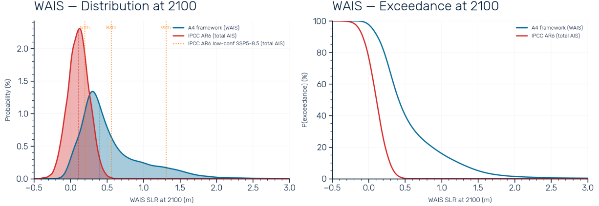
Figure S8: WAIS endpoint distributions and exceedance probabilities: A4 vs IPCC. Left: probability density at 2100 for the A4 WAIS framework (blue) compared with the IPCC AR6 total Antarctic projection (red). The A4 distribution is wider, with a higher median and a heavier right tail arising from the MISI skewness and rheology correction. Right: exceedance probability curves, showing that the A4 framework assigns substantially higher probability to exceeding any given threshold above \sim 0.1 m. The IPCC distribution assigns near-zero probability to outcomes exceeding 0.5 m, whereas the A4 framework assigns \sim 40\% probability to this threshold.
