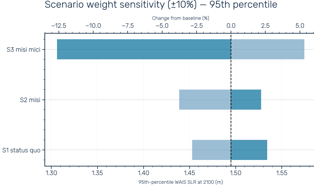
Figure S10: Scenario weight sensitivity—95th percentile. As in Fig. S11, but for the 95th percentile (5% exceedance) of the WAIS SLR distribution at 2100. The upper axis shows the percentage change from the baseline value ( \sim 1.5 m). The tail of the distribution is similarly insensitive to weight perturbations, with the largest shift ( \sim \pm 12\% from S3) remaining a small fraction of the total.
