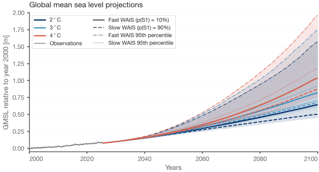
Figure 9: Global mean sea-level projections. Global mean sea level relative to 2000 under 2 °C (SSP1-2.6), 3 °C (SSP2-4.5), and 4 °C (SSP3-7.0) of warming, with satellite altimetry observations (grey) ( Beckley et al. , 2017). The ‘fast WAIS’ scenario makes accelerated WAIS mass loss very likely ( p(S1) = 10\% ), while the ‘slow WAIS’ scenario makes continued mass loss along the observed trajectory very likely ( p(S1) = 90\% ). Solid lines show the fast WAIS forecast median with its 90% CI (5–95th percentile, shaded). Dashed lines show the slow WAIS median. Dash-dot and dotted lines mark the 95th percentile of the fast and slow WAIS forecasts, respectively.
