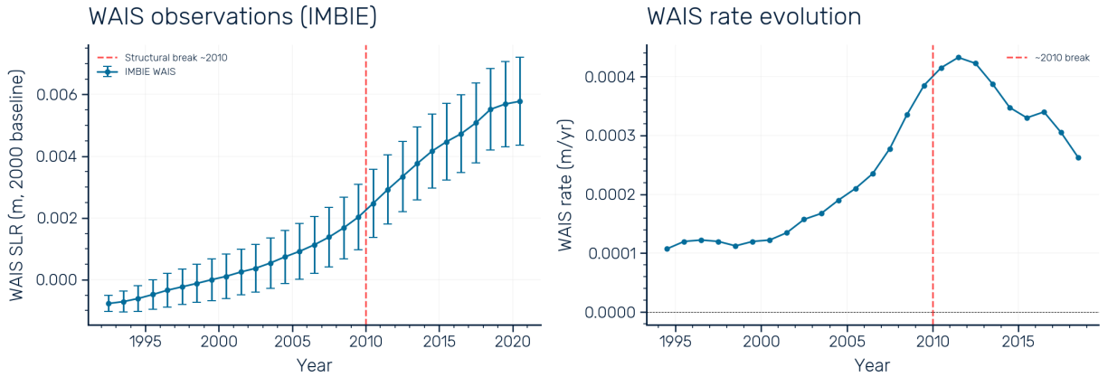
Figure 9: WAIS observational record. Left: cumulative WAIS sea-level contribution from IMBIE (1992–2020; [16]) with measurement uncertainties, relative to the year-2000 baseline. The structural break at \sim 2010 (red dashed line) separates a period of acceleration from apparent deceleration. Right: WAIS mass loss rate evolution, showing the rate increasing from \sim 0.15 \text{ mm yr}^{-1} in the early 1990s to a peak of \sim 0.44 \text{ mm yr}^{-1} around 2010–2012, followed by a decline that may reflect internal ocean variability in the Amundsen Sea [36].
