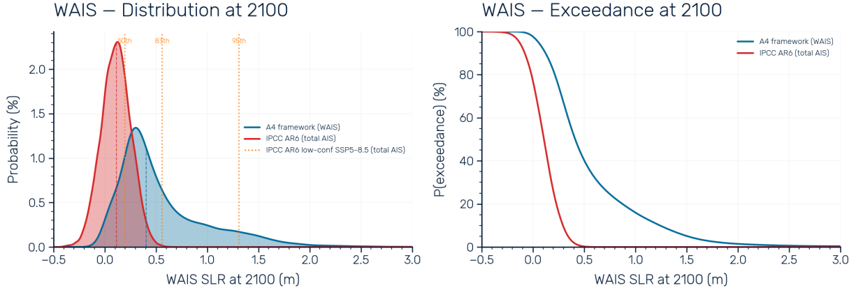
Figure 10: WAIS endpoint distributions and exceedance probabilities: A4 vs IPCC. Left: probability density at 2100 for the A4 WAIS framework (blue) compared with the IPCC AR6 total Antarctic projection (red). The A4 distribution is wider, with a higher median and a heavier right tail arising from the MISI skewness and rheology correction. Right: exceedance probability curves, showing that the A4 framework assigns substantially higher probability to exceeding any given threshold above \sim 0.1 m. The IPCC distribution assigns near-zero probability to outcomes exceeding 0.5 m, whereas the A4 framework assigns \sim 40\% probability to this threshold.
