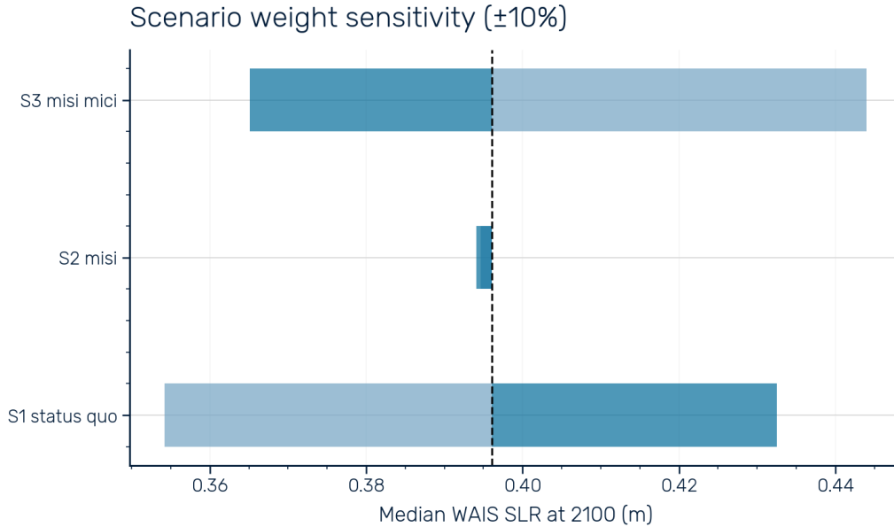
Figure 11: Scenario weight sensitivity. Tornado plot showing the effect of \pm 10 percentage-point perturbations to each scenario weight on the median WAIS SLR at 2100. Dark bars show the inner perturbation range; light bars extend to the full \pm 10\% range. The dashed vertical line indicates the baseline median (0.40 m). The mixture median is insensitive to weight perturbations, varying by less than 0.09 m across all perturbations—small relative to the 90% credible interval of the mixture distribution ( \sim 1.4 m).
