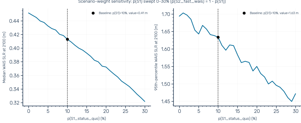
Figure S5: Scenario weight sensitivity. Median (left) and 95th-percentile (right) WAIS SLR at 2100 as a function of P(S1\_status\_quo) , swept from 0 to 30% ( P(S2\_fast\_wais) = 1 - P(S1) ). The marker indicates the baseline value ( P(S1) = 0.10 ). Both statistics vary only modestly across the swept range, confirming that within-scenario uncertainty dominates over the assigned scenario weight.
