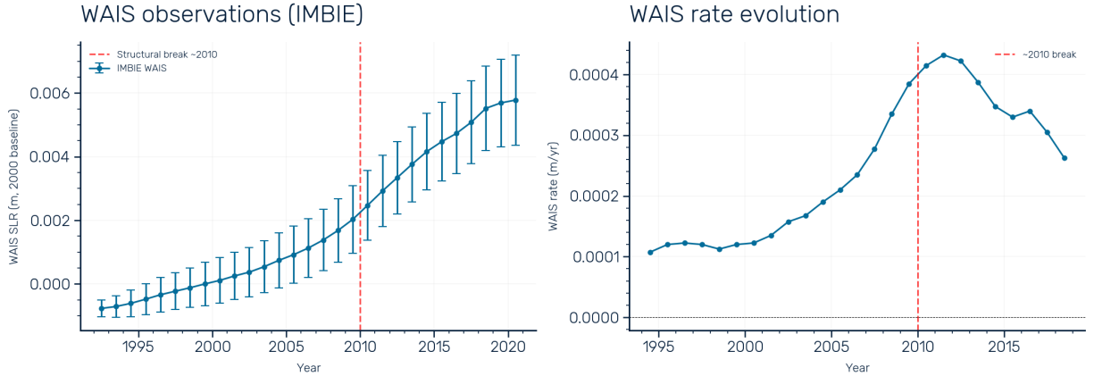
Figure S3: WAIS observational record. Left: cumulative WAIS sea-level contribution from IMBIE (1992–2020; Otosaka et al. , 2023) with measurement uncertainties, relative to the year-2000 baseline. The structural break at \sim 2010 (red dashed line) separates a period of acceleration from apparent deceleration. Right: WAIS mass loss rate evolution, showing the rate increasing from \sim 0.15 mm yr ^{-1} in the early 1990s to a peak of \sim 0.44 mm yr ^{-1} around 2010–2012, followed by a decline that may reflect internal ocean variability in the Amundsen Sea ( Jenkins et al. , 2018).
