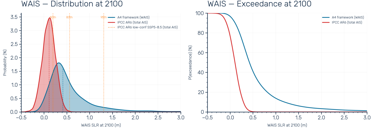
Figure S4: WAIS endpoint distributions and exceedance probabilities: A4 vs IPCC. Left: probability density at 2100 for the A4 WAIS framework (blue) compared with the IPCC AR6 total Antarctic projection (red). The A4 distribution is wider, with a higher median and a heavier right tail arising from the MISI skewness and rheology correction. Right: exceedance probability curves, showing that the A4 framework assigns substantially higher probability to exceeding any given threshold above \sim 0.1 m. The IPCC distribution assigns near-zero probability to outcomes exceeding 0.5 m, whereas the A4 framework assigns \sim 40\% probability to this threshold.
