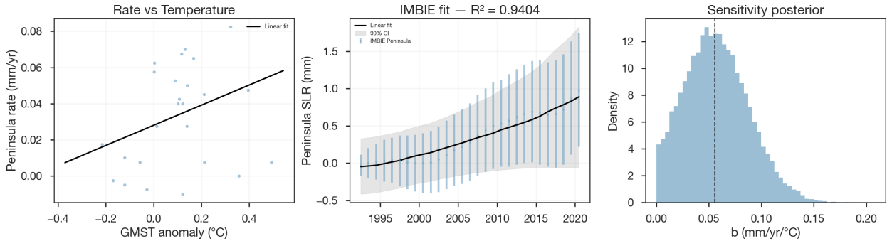
Figure S2: Peninsula model diagnostics. (a) Peninsula mass loss rate vs GMST anomaly with the fitted linear relationship. (b) Cumulative Peninsula SLR: IMBIE observations with the model fit and 90% credible interval; R^2 = 0.94 . (c) Posterior distribution for the temperature sensitivity b .
