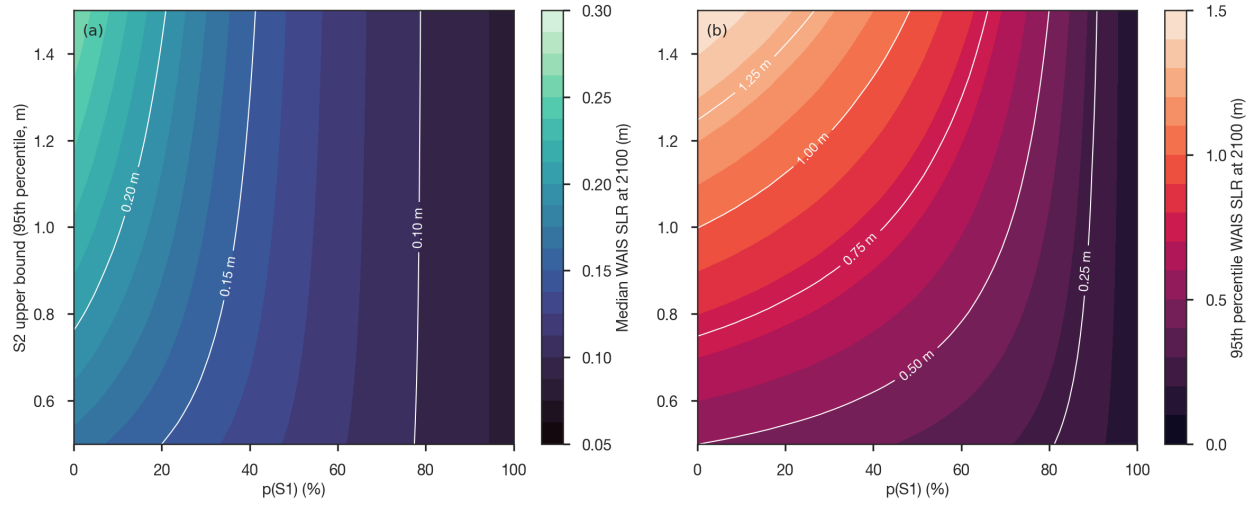
Figure 8: WAIS contribution to GMSL at 2100 as a function of the two mixture parameters. (a) Median and (b) 95th percentile of the S1/S2 mixture (relative to 2000) across the S1 probability, p(S1) , and the S2 upper bound (95th percentile of S2 at 2100).
