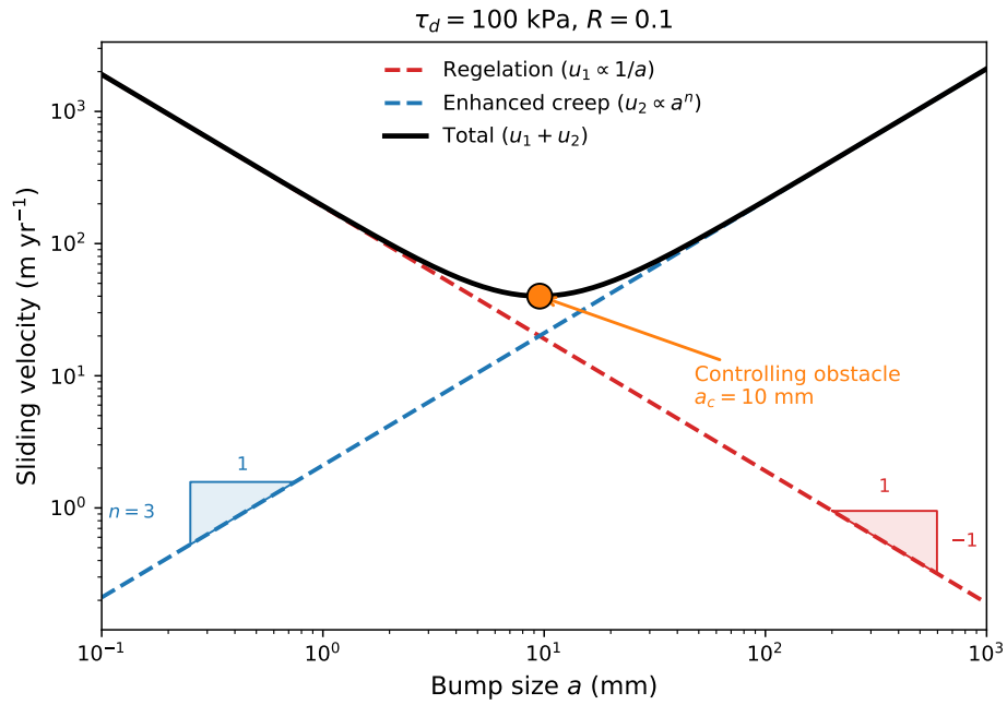
Figure 2: Sliding velocity contributions from regelation ( u_1 \propto 1/a ) and enhanced creep ( u_2 \propto a^n ) as functions of bump size a for \tau_d = 100 kPa and roughness R = 0.1 . The controlling obstacle size a_c (orange circle) is the bump size at which the total velocity u_1 + u_2 is minimized; bumps of this size provide the greatest resistance to sliding.
