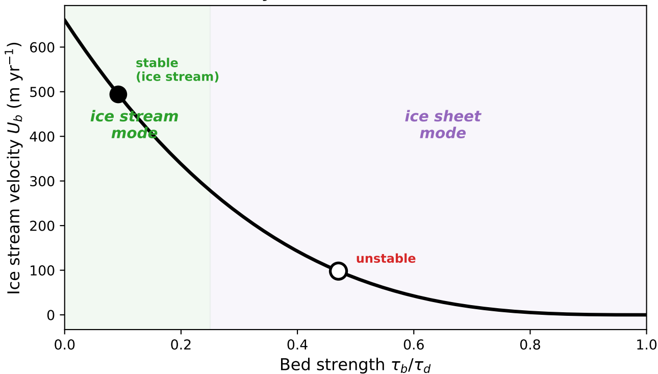
(b) Ice stream velocity
