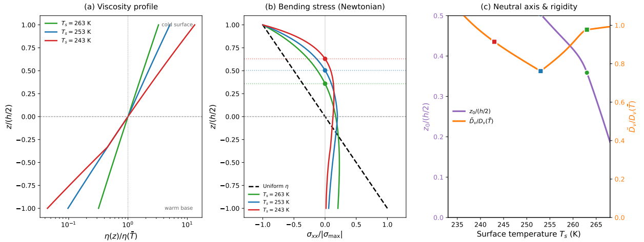
Figure 11: Effect of depth-dependent temperature on viscous beam bending, for a linear temperature profile with T_b = 273 K and varying surface temperature T_s . (a) Viscosity profile \eta(z)/\eta(\bar{T}) : the surface-to-base contrast ranges from \sim 10 ( T_s = 263 K) to \sim 500 ( T_s = 243 K). (b) Newtonian bending stress \sigma_{xx}(z) (normalized by the surface value) for uniform \eta (dashed black) and depth-dependent \eta (solid curves). The neutral axis (horizontal dotted lines) shifts toward the cold surface. (c) Neutral axis position z_0/(h/2) and effective rigidity ratio \tilde{D}_v/D_v(\bar{T}) as functions of T_s . Colder surface temperatures produce larger asymmetry and greater rigidity reduction. All quantities are for the beam (uniaxial) case.
