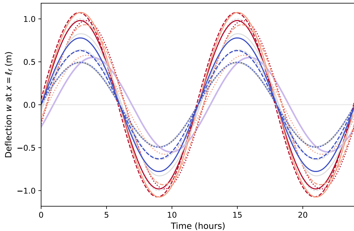
(d) Time series at x = \ell_f = 2.6 km
