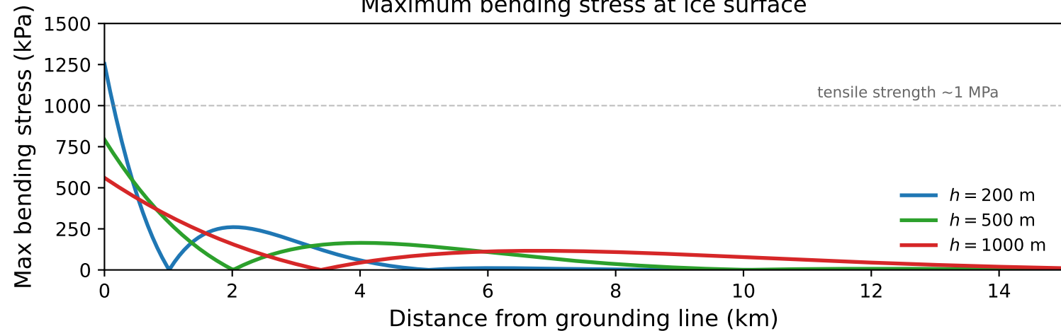
Maximum bending stress at ice surface
