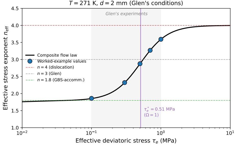
Figure 6: Effective stress exponent n_{\text{eff}} as a function of stress at Glen’s experimental conditions ( T = 271 K, d = 2 mm). The five points correspond to the values computed in the table above. The crossover stress \tau_e^* \approx 0.51 MPa, where dislocation creep and GBS-accommodated basal slip contribute equally ( \Omega = 1 ), is marked by a vertical line. Glen’s experimental stress range is shaded.
