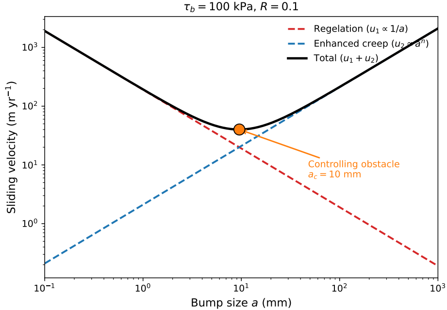
Figure 2: Sliding velocity contributions from regelation ( u_1 \propto 1/a ) and enhanced creep ( u_2 \propto a^n ) as functions of bump size a for \tau_b = 100 kPa and roughness R = 0.1 . The controlling obstacle size a_c (orange circle) is the bump size at which the total velocity u_1 + u_2 is minimized; bumps of this size provide the greatest resistance to sliding.
