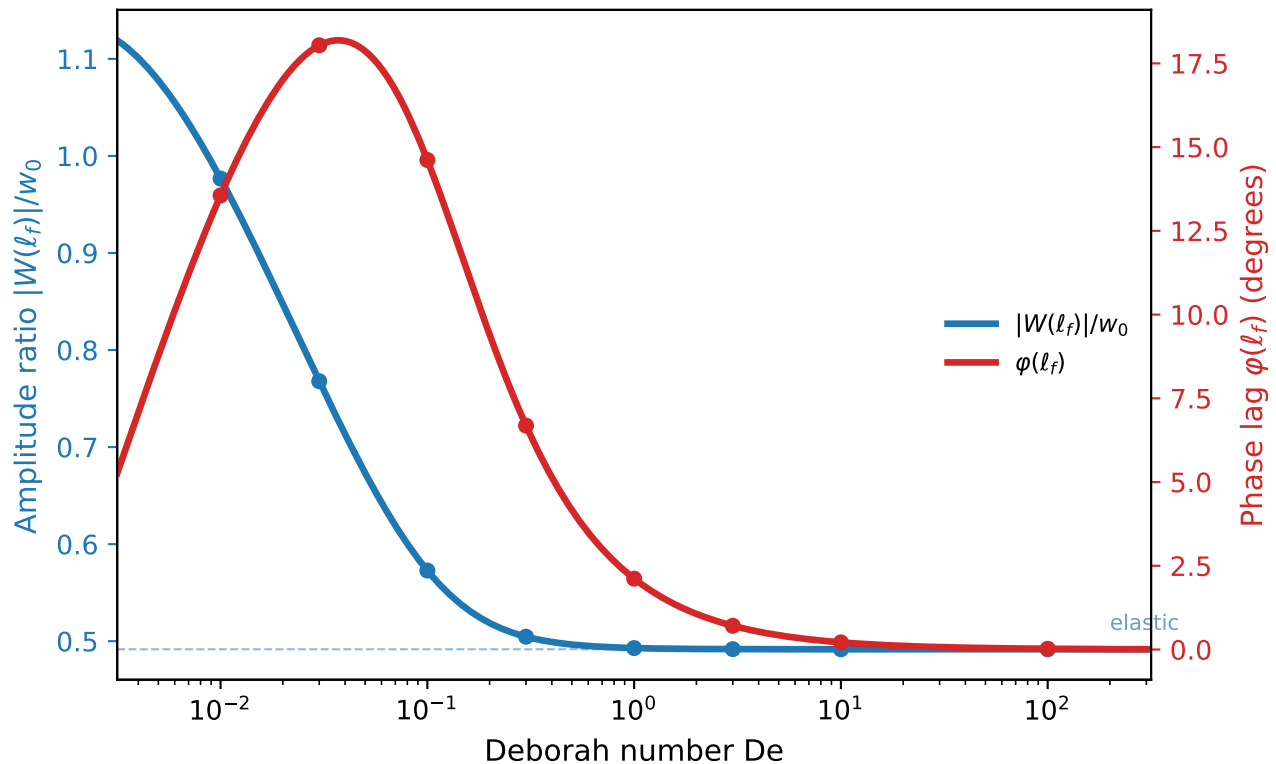
(b) Amplitude and phase at x = \ell_f
