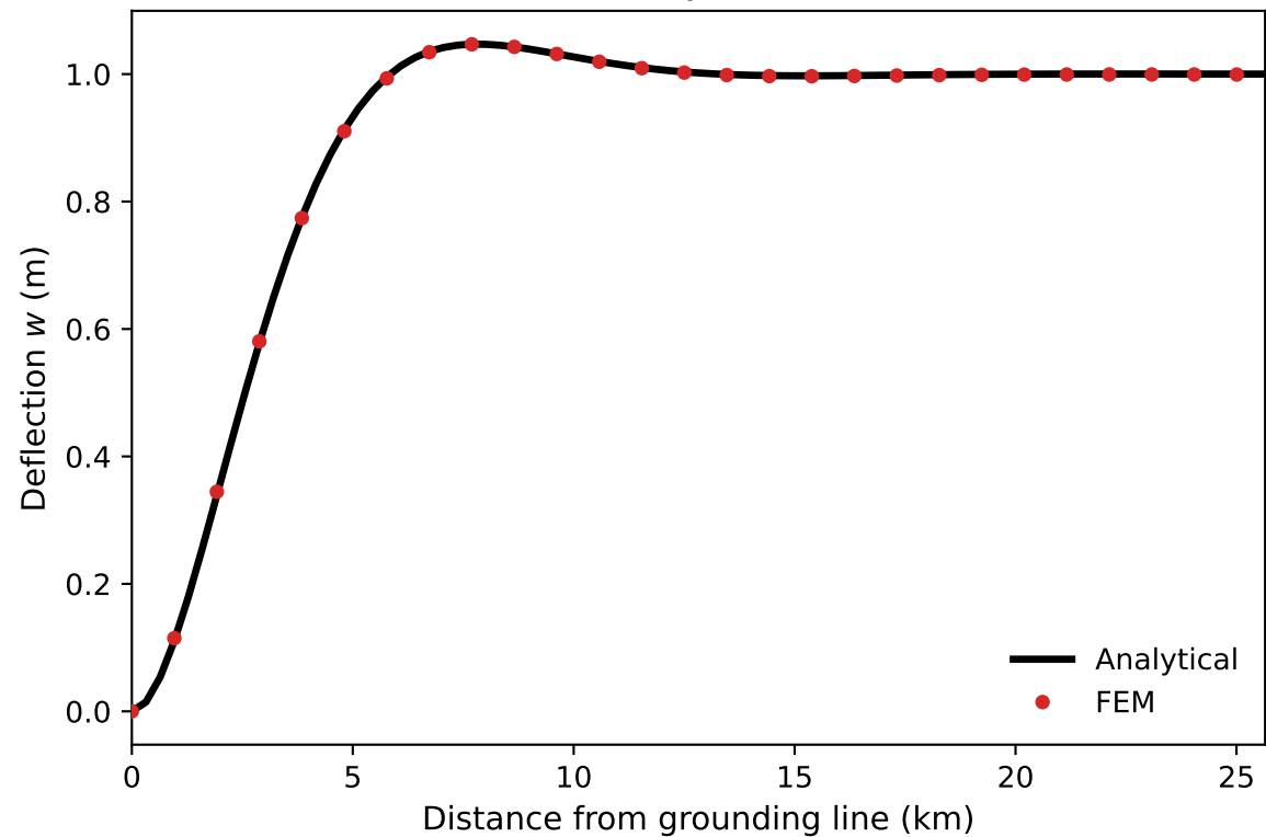
(a) FEM vs analytical, De = 0.30
