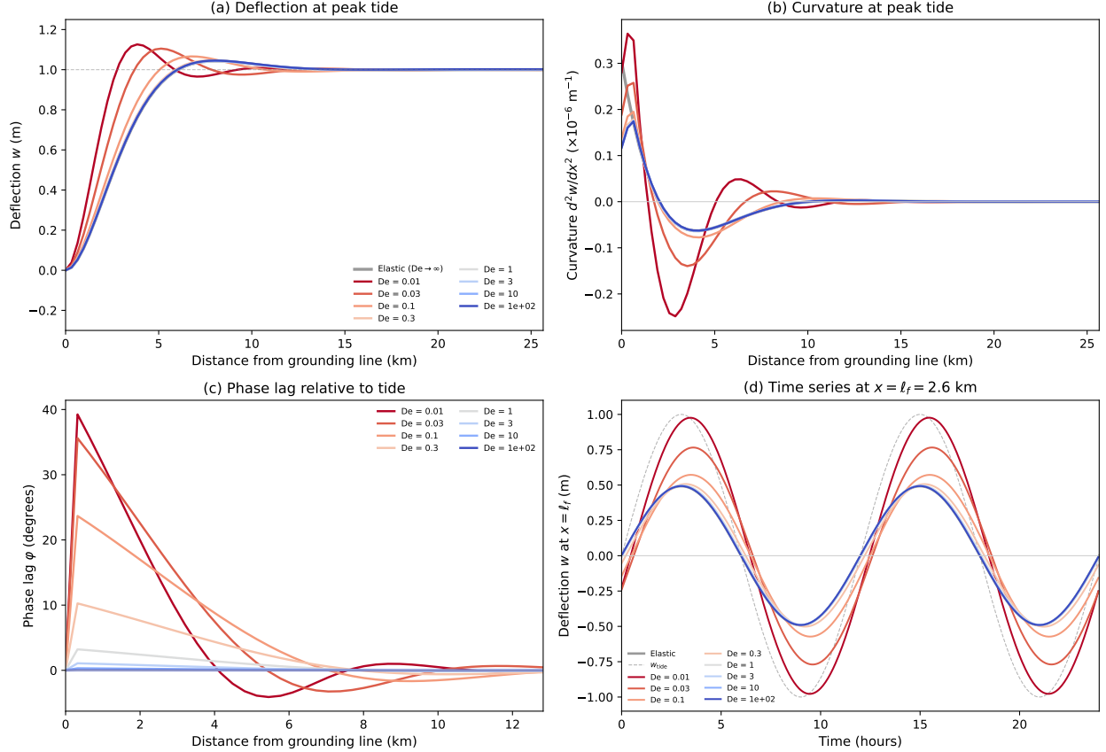
Figure 12: Maxwell viscoelastic tidal flexure at a grounding zone ( h = 500 \text{ m} , w_0 = 1 \text{ m} , T_{\text{tide}} = 12 \text{ hr} ), solved numerically for Deborah numbers from De = 0.01 (viscous limit, warm colors) to De = 100 (elastic limit, cool colors). (a) Deflection profiles at peak tide. (b) Curvature profiles. (c) Phase lag \phi(x) relative to the tidal forcing (from the analytical Newtonian solution). (d) Time series of deflection at x = \ell_f . The black curves show the elastic reference ( De \rightarrow \infty ). As De increases, the response transitions continuously from the broad, phase-shifted viscous solution to the narrow, in-phase elastic solution.
