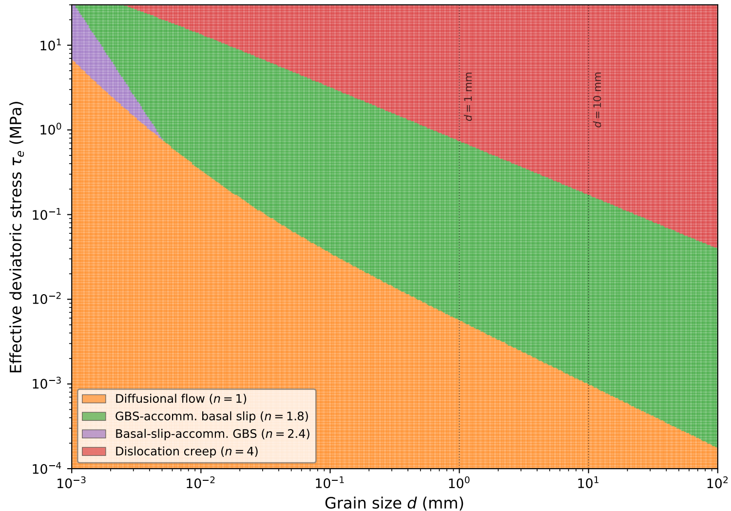
Deformation mechanism map ( T = 263\text{ K} )
