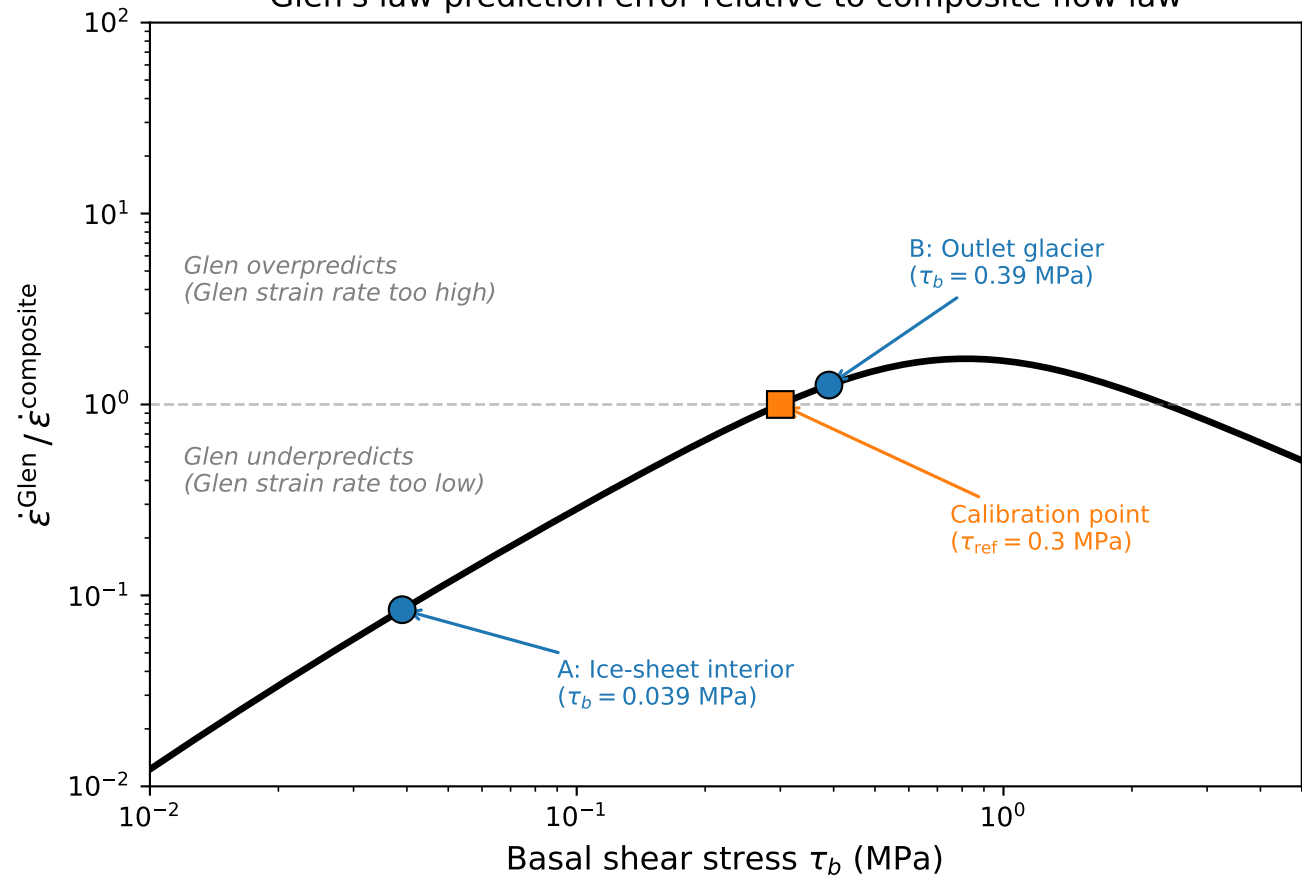
Glen's law prediction error relative to composite flow law
